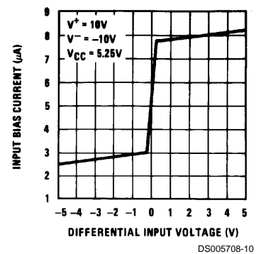
Input Characteristics
