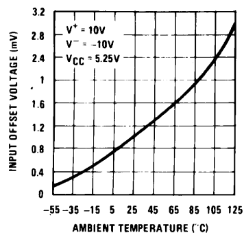
Offset Voltage
