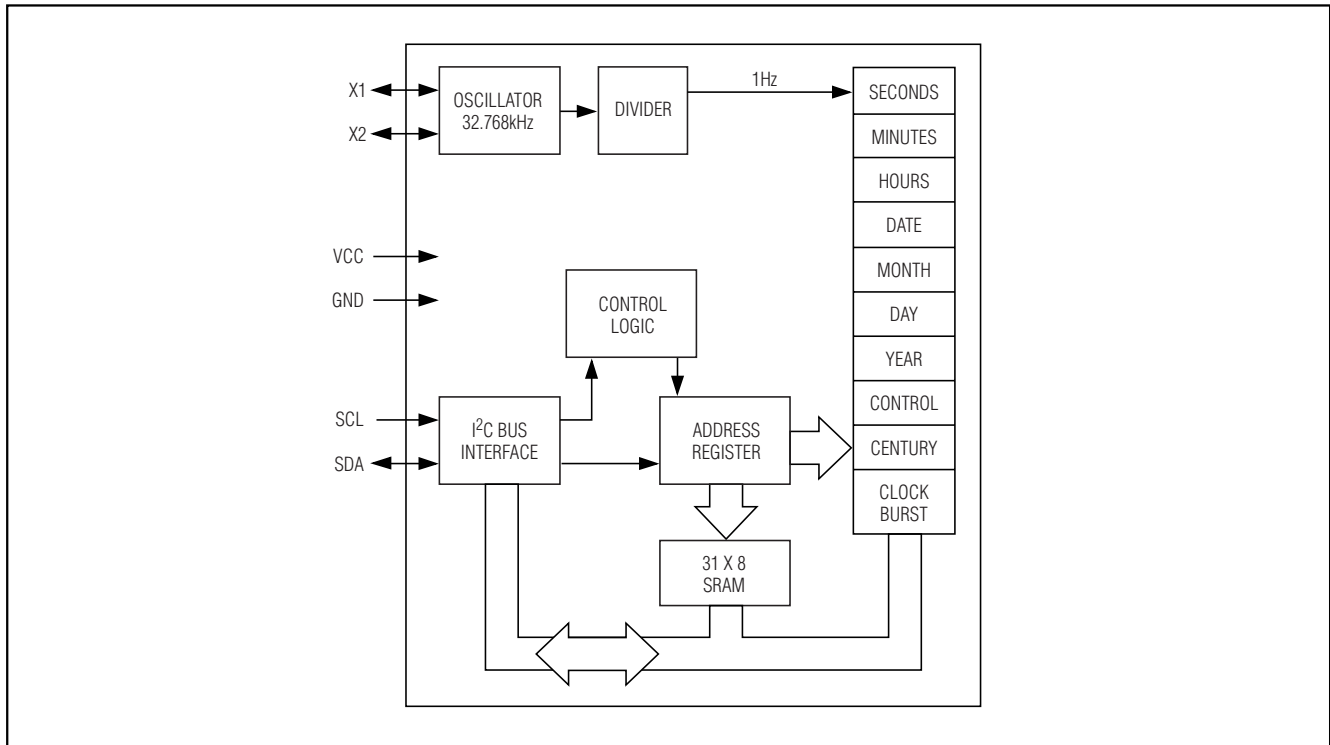
Figure 2. Functional Diagram
