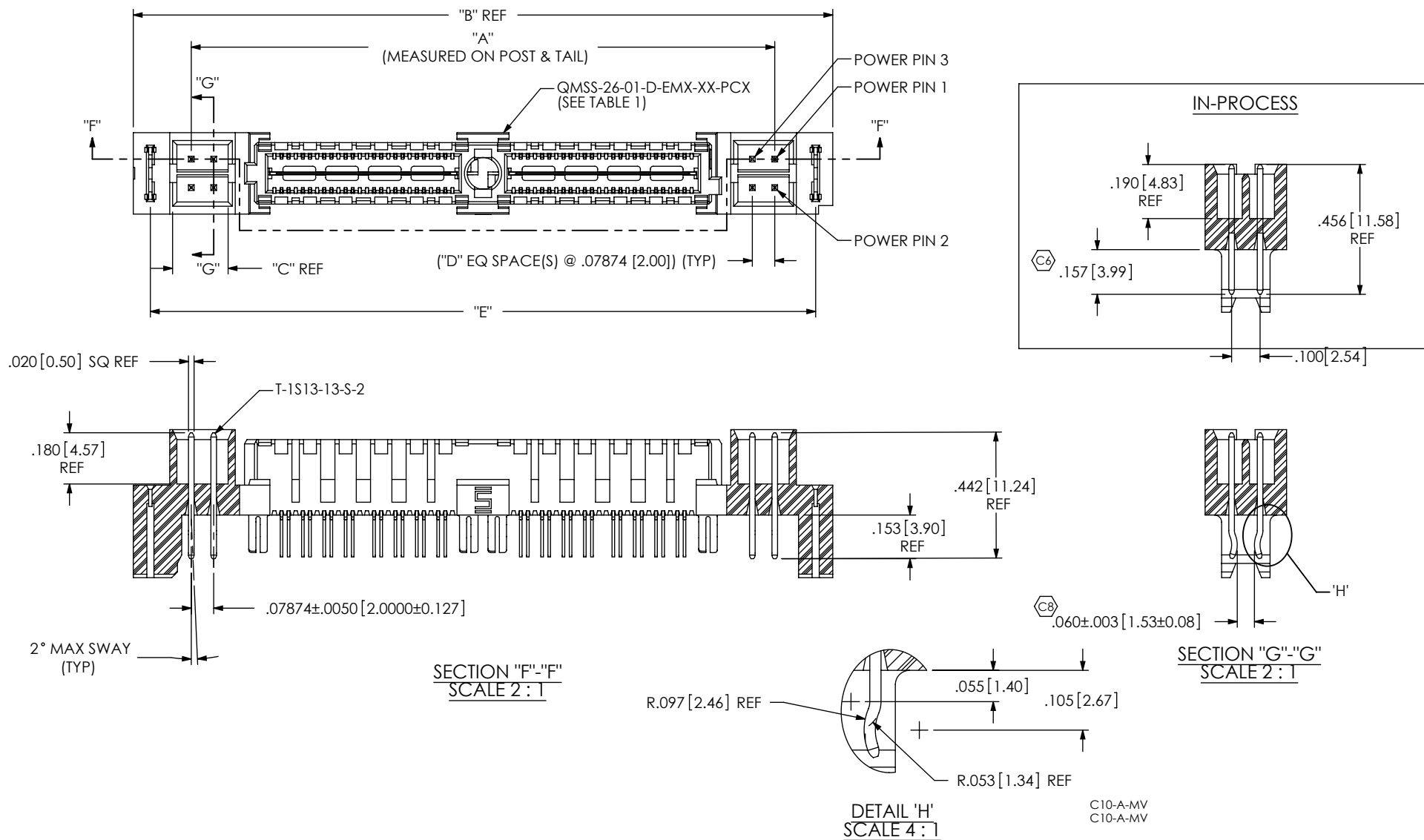
FIG. 2 -PCX OPTION QMS-032-01-X-D-DP-EM2-PC4 SHOWN [DIFFERENT AS SHOWN, OTHERWISE SAME AS FIG. 1]
