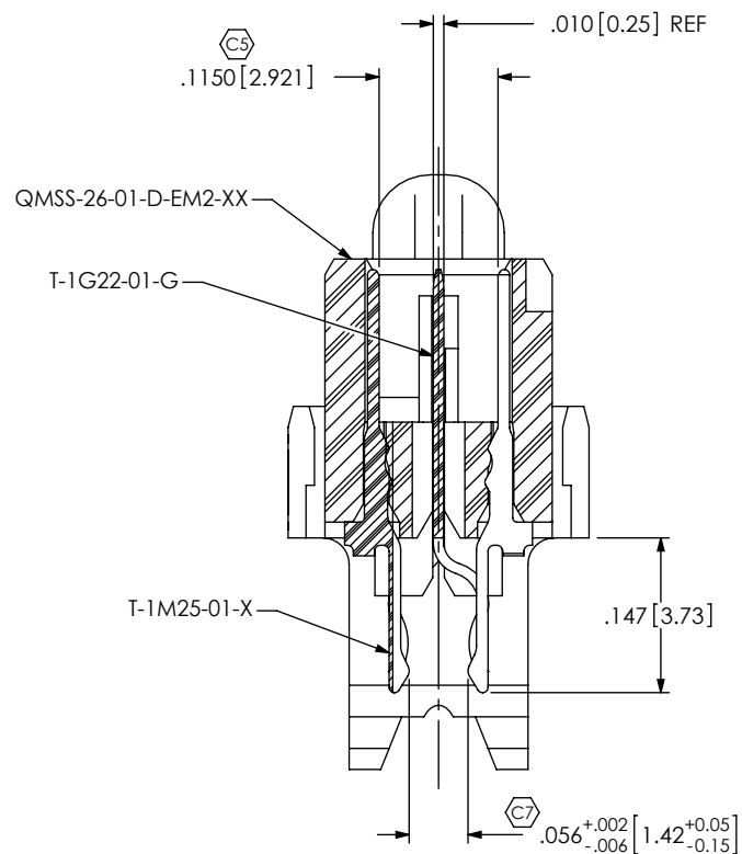
SECTION "A"-"A" SCALE 5:1
