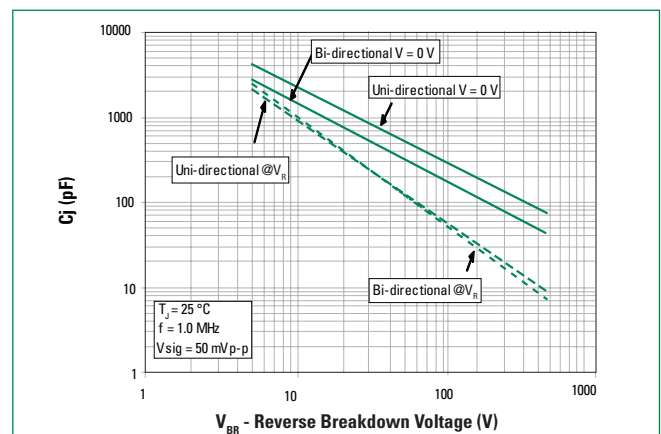
Figure 6 - Typical Junction Capacitance @ Standard Product
