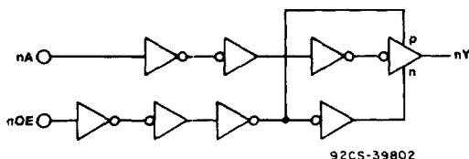
Fig. 1 - Logic Diagram
