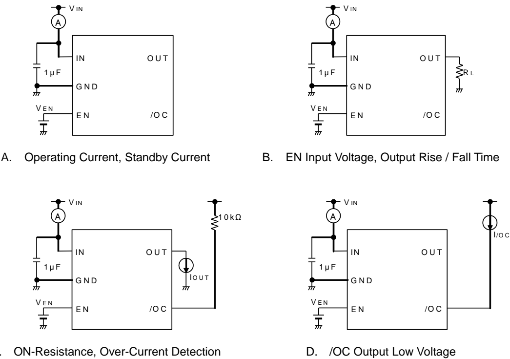
Figure 1. Measurement Circuit
