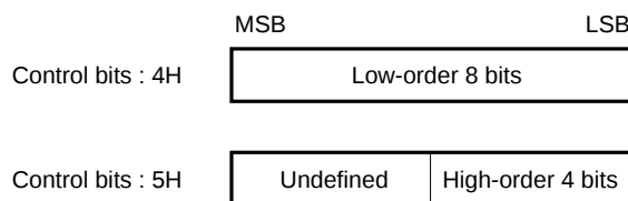
Fig. 2-3 Lock Address Format
