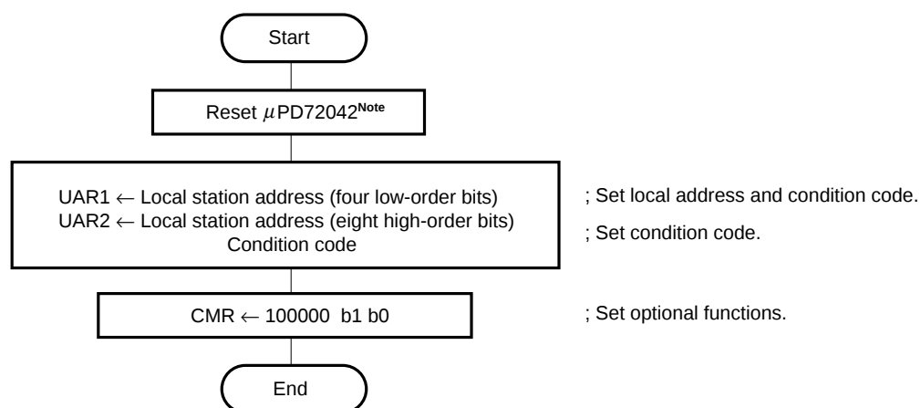
Fig. 6-4 \mu PD72042 Initial Setting Routine
