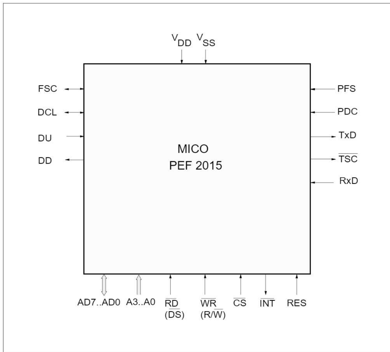
Figure 2 Logic Symbol
