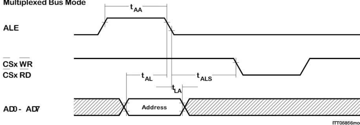
Figure 19 a Siemens/Intel Bus Mode
