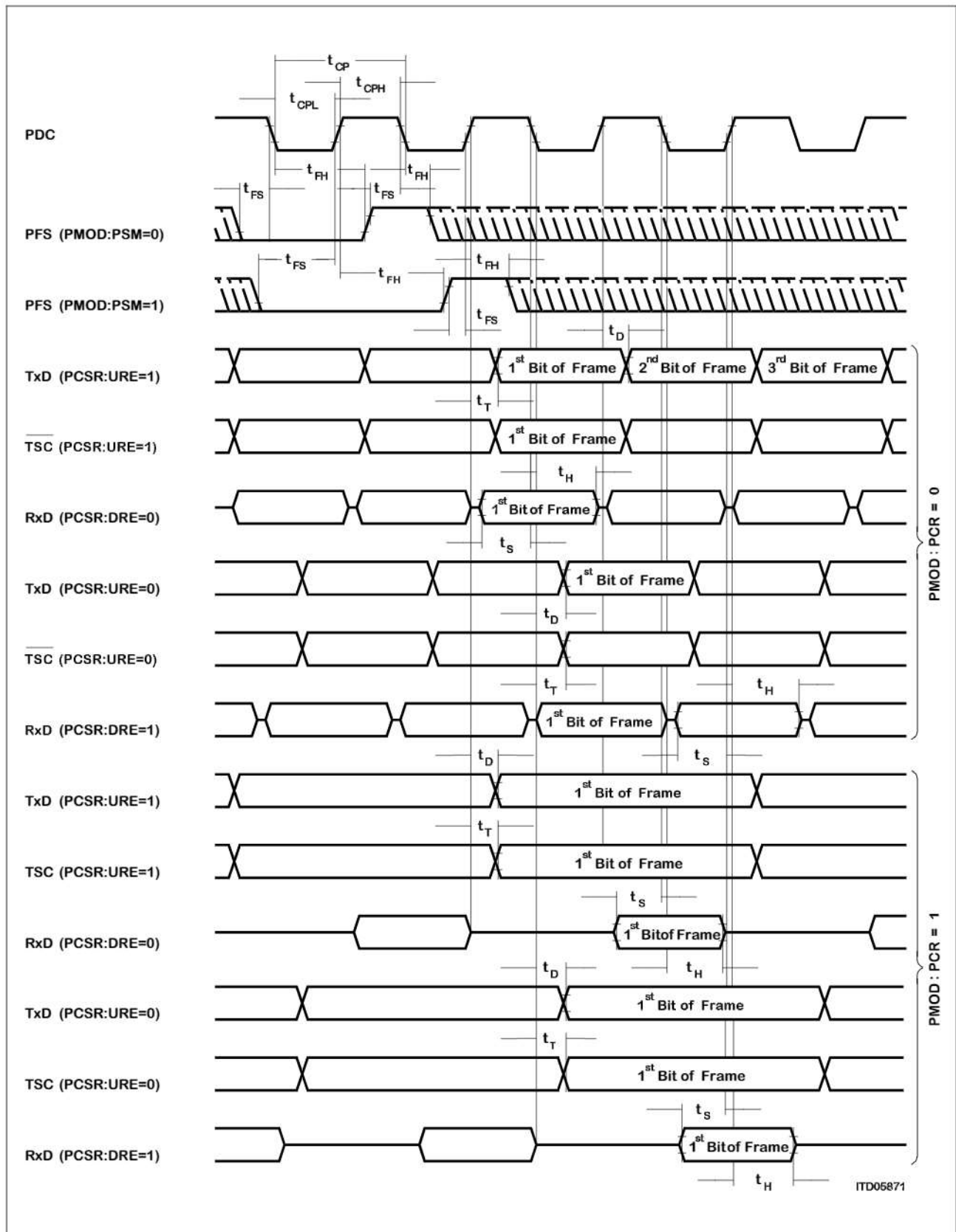
Figure 24 PCM-Interface Timing
