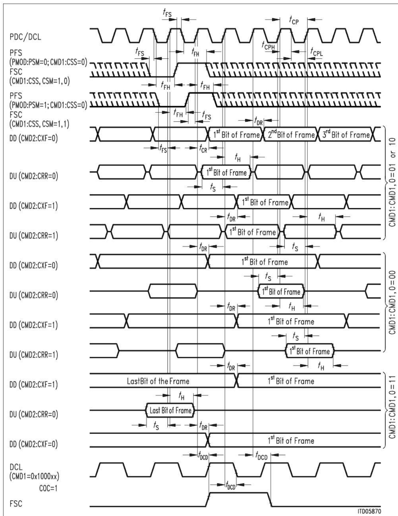
Figure 23 Configurable Interface Timing, CMD:CSP1,0 = 00 (prescaler divisor = 2)
