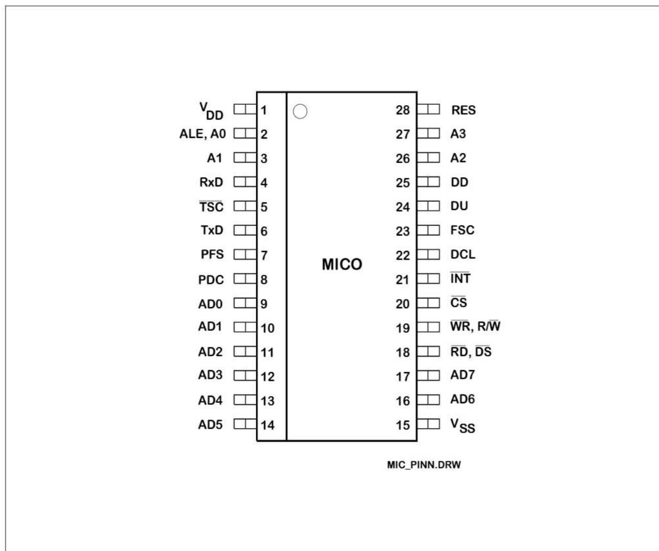
Figure 1 Pinning Diagram
