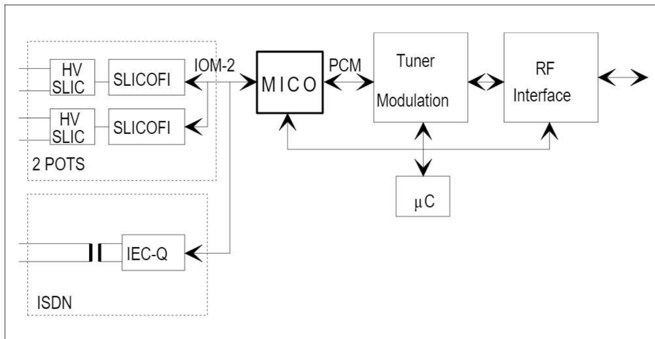
Figure 16 Example using the MICO in an UE
