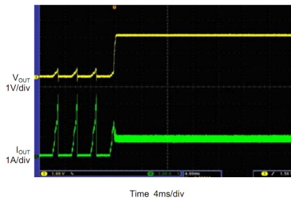
Fig. 15: Short Circuit Recovery V_{IN}=3.3V , V_{OUT}=2.5V
