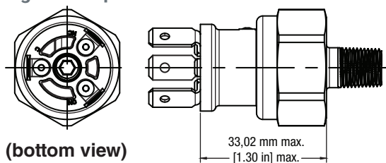
Figure 25. Spade terminal
