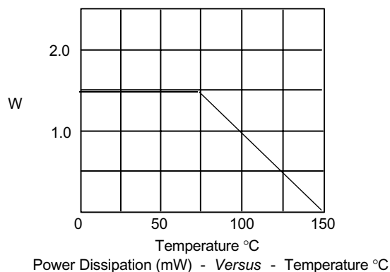
Figure 2 - Derating Curve
