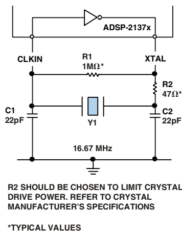
Figure 6. 266 MHz Operation (Fundamental Mode Crystal)
