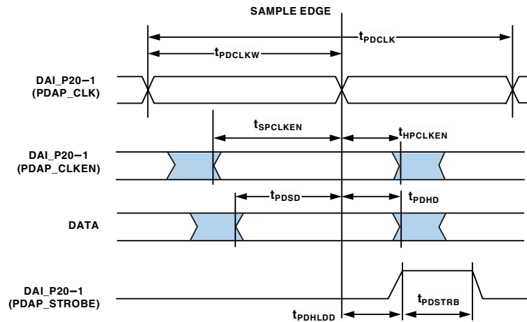
Figure 22. PDAP Timing
