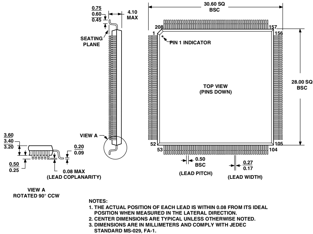
Figure 40. 208-Lead Metric Quad Flat Package [MQFP] (S-208-2)
