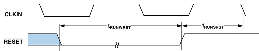
Figure 7. Reset
