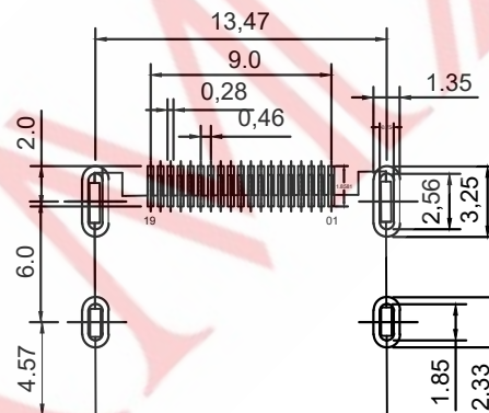
RECOMMEND PCB LAYOUT( \pm 0.05 )
