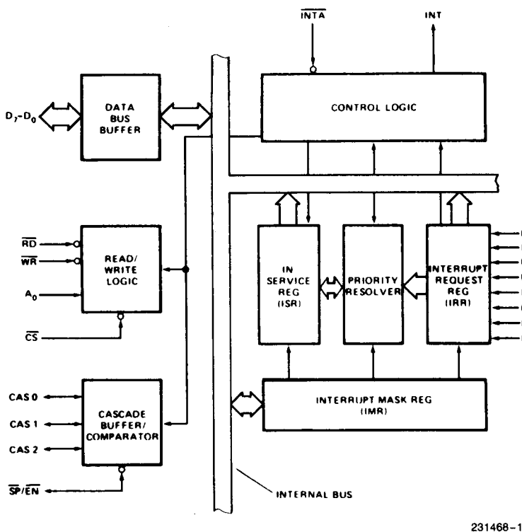
Figure 1. Block Diagram
