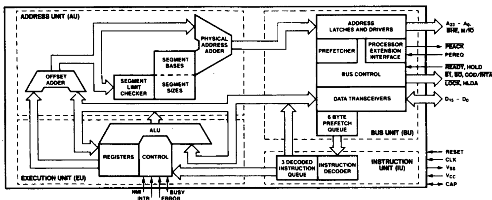
Figure 1. 80C286 Internal Block Diagram
