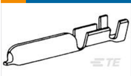
TE Part #62074-1 PIN .125 (3.17 MM) 24-20 AWG 0.42 BR
