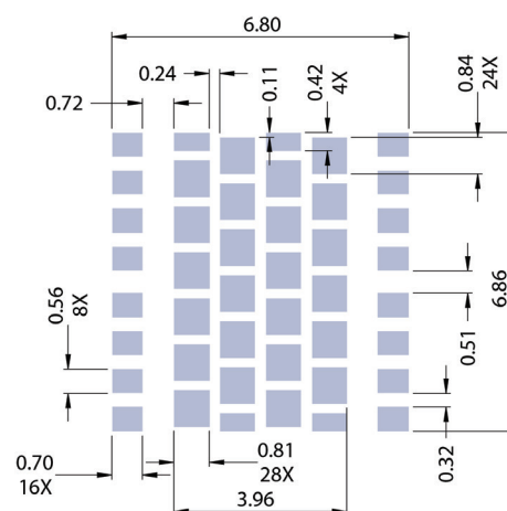
Recommended 3-V, 6-V & 12-V Stencil Openings
