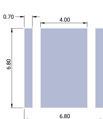
Recommended 3-V PCB Footprint
