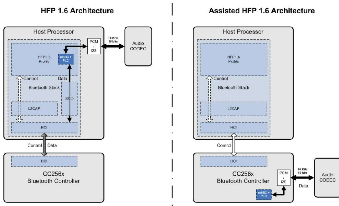
Figure 6-15. HFP 1.6 Architecture Versus Assisted HFP 1.6 Architecture
