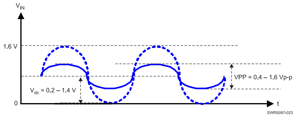
Figure 6-5. External Fast Clock (Sine Wave, DC-Coupled)
