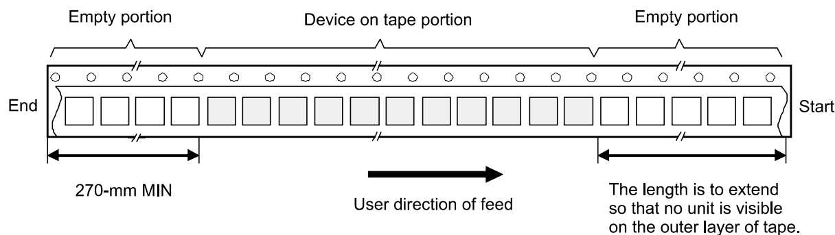
Figure 9-2. Carrier Tape and Pockets
