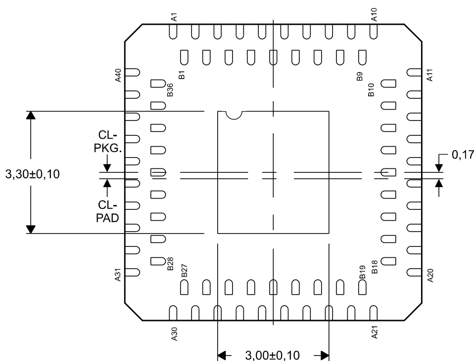
Bottom View
