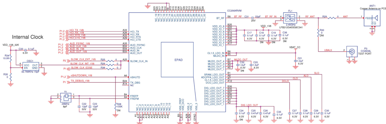
Figure 7-1. Reference Schematics
