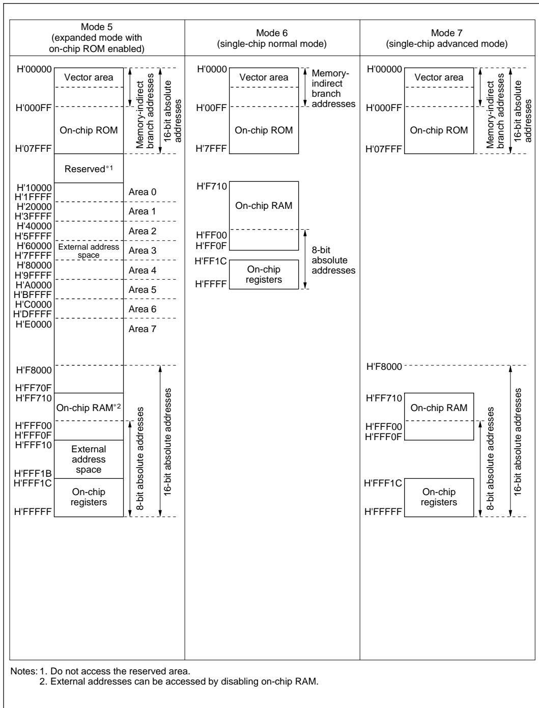
Figure 3-3 H8/3040 Memory Map in Each Operating Mode (2)
