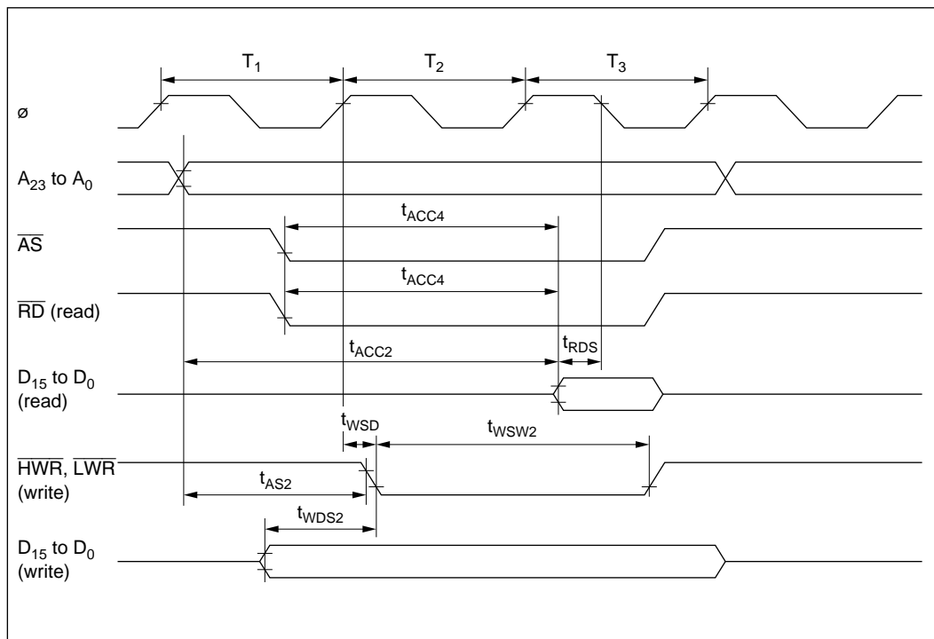
Figure 20-5 Basic Bus Cycle: Three-State Access
