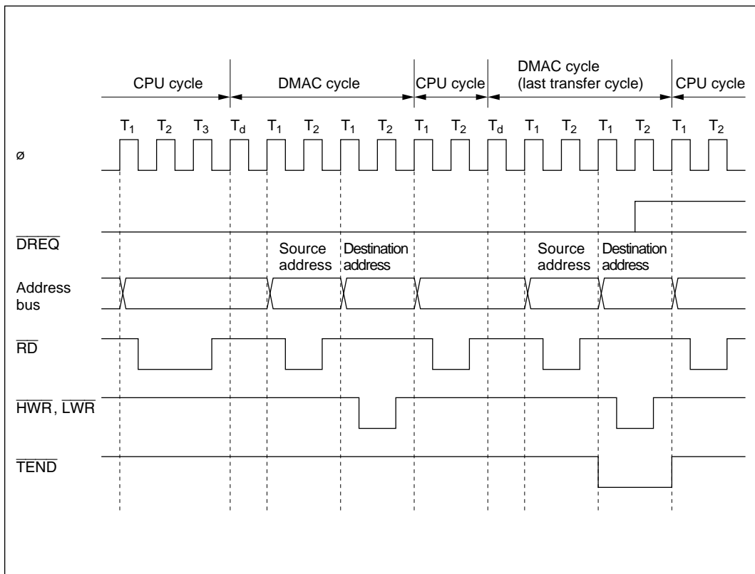
Figure 8-14 Bus Timing of DMA Transfer Requested by Low \overline{DREQ} Input
