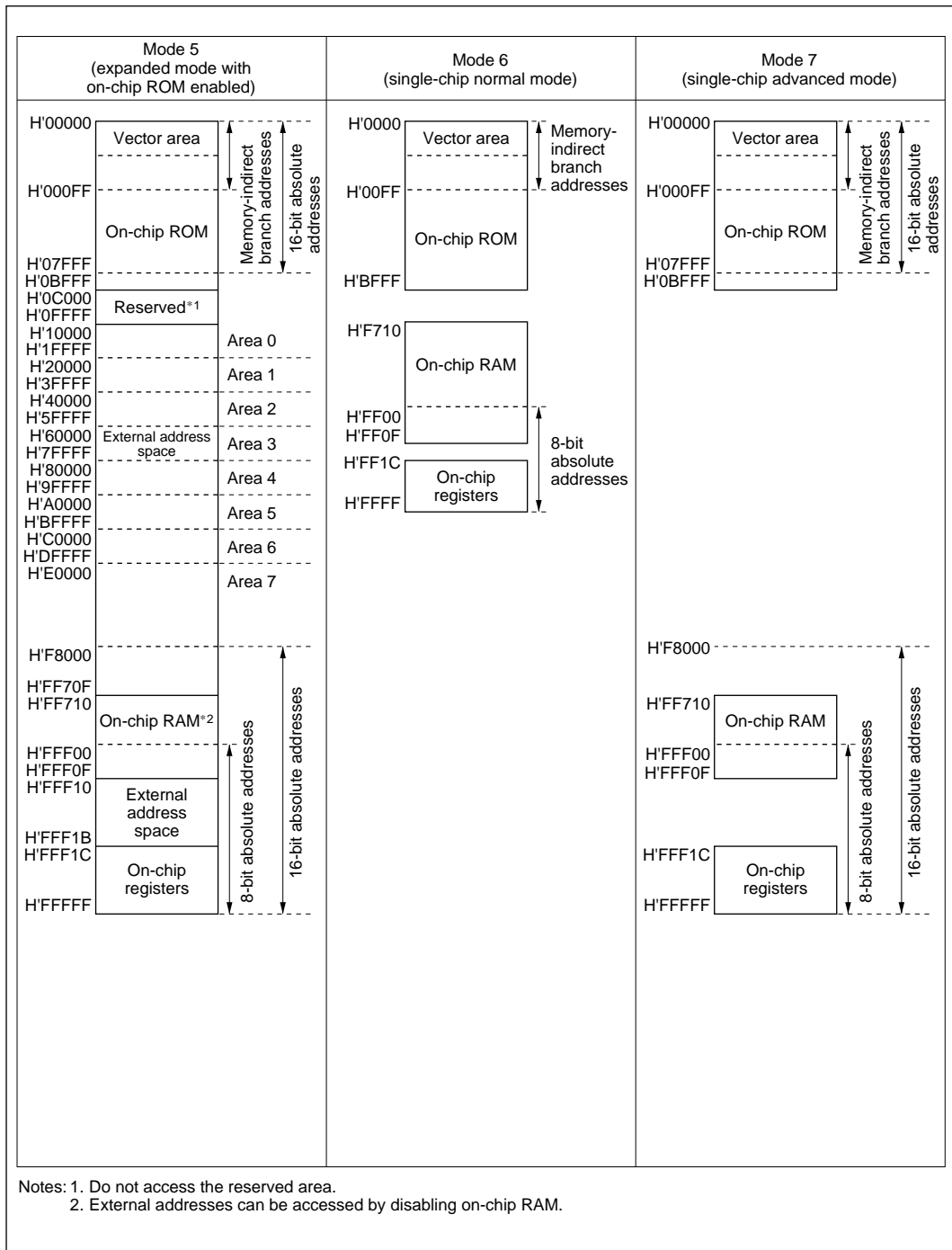
Figure 3-2 H8/3041 Memory Map in Each Operating Mode (2)
