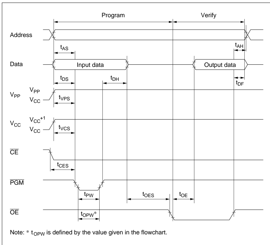
Figure 17-5 PROM Program/Verify Timing
