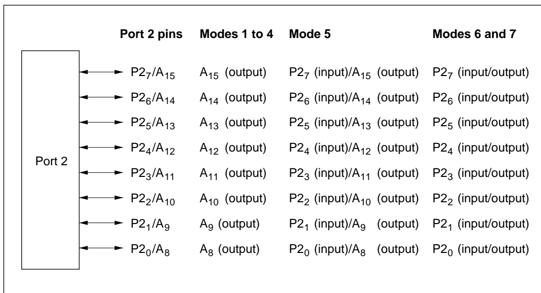
Figure 9-5 Port 2 Pin Configuration
