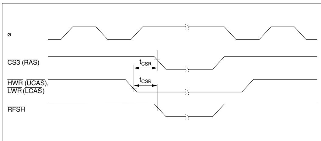
Figure 20-12 DRAM Bus Timing (Self-Refresh Mode) — 2CAS Mode —
