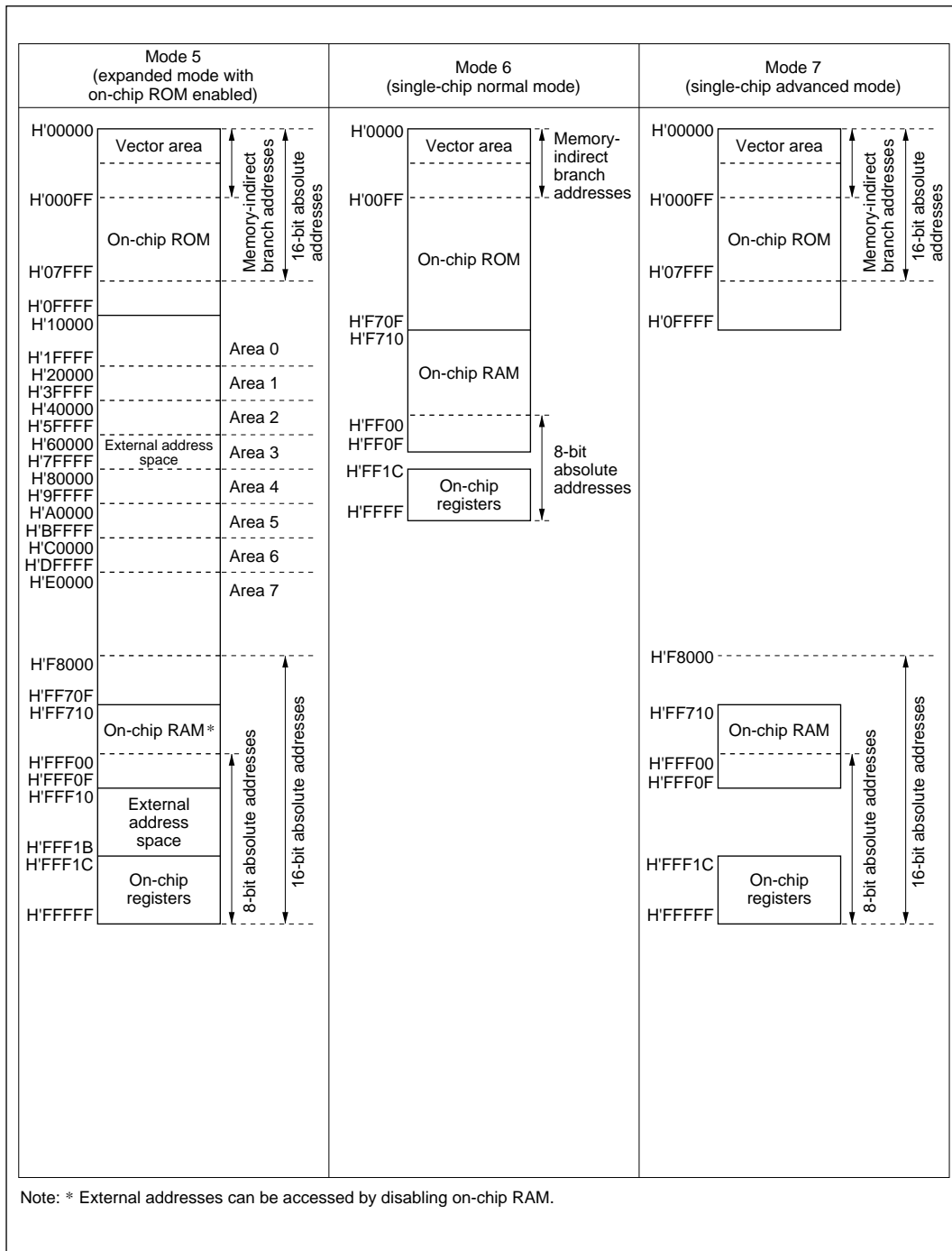
Figure 3-1 H8/3042 Memory Map in Each Operating Mode (2)
