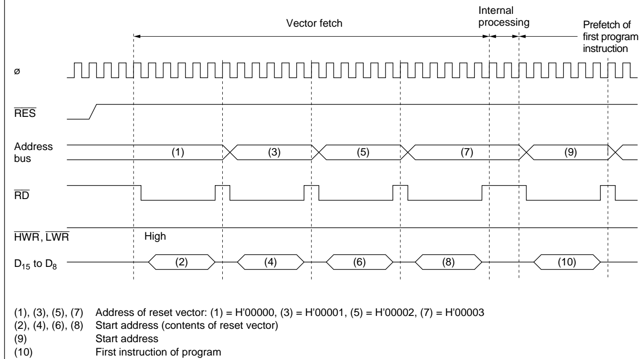
Figure 4-2 Reset Sequence (Modes 1 and 3)
