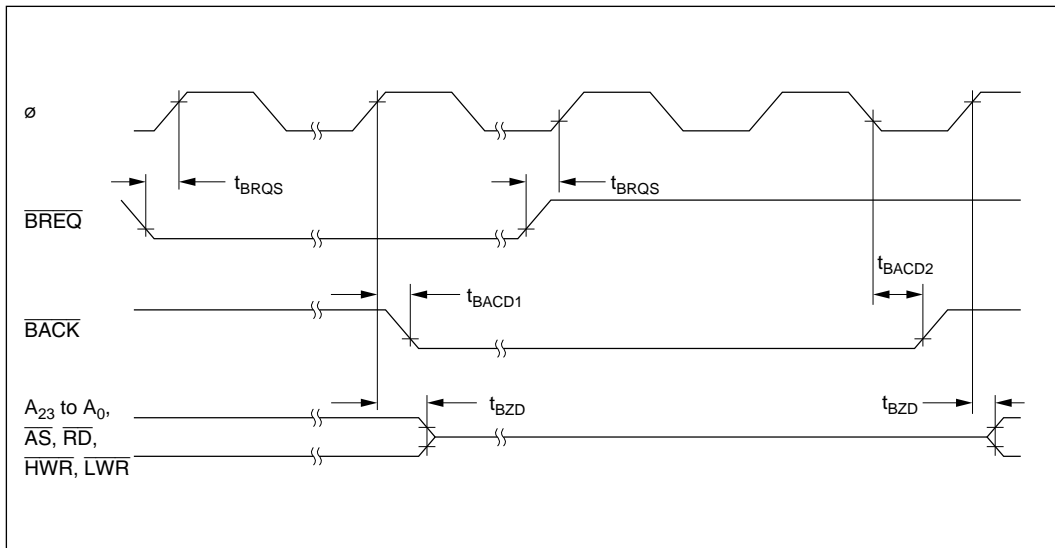
Figure 20-18 Bus-Release Mode Timing
