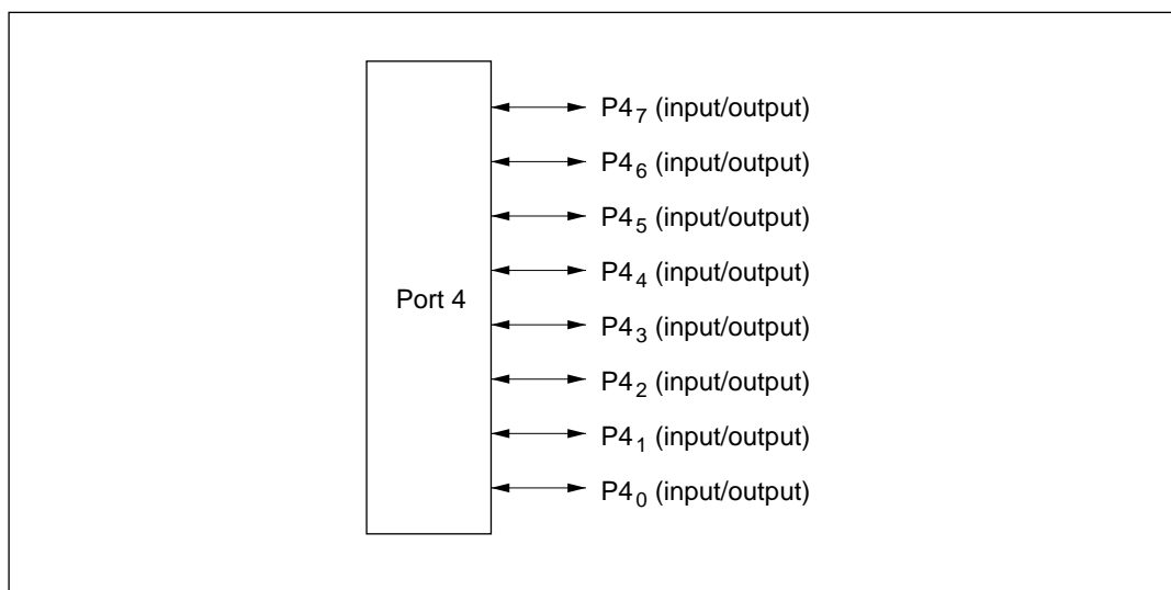
Figure 9-15 Pin Functions in Modes 6 and 7 (Port 4)
