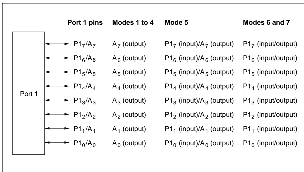
Figure 9-1 Port 1 Pin Configuration
