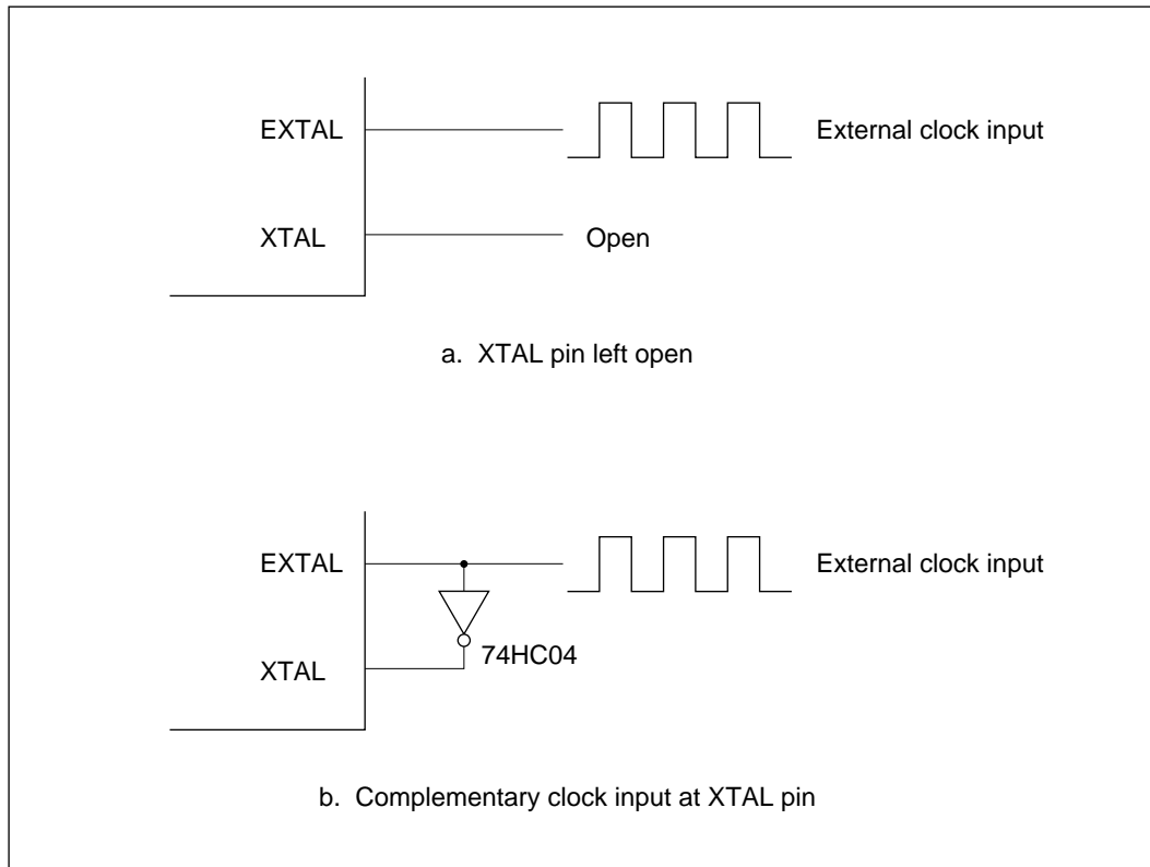
Figure 18-5 External Clock Input (Examples)
