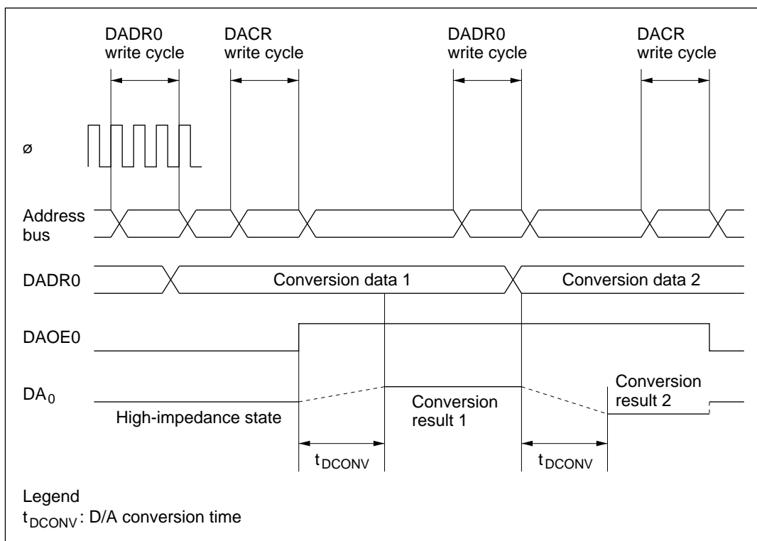
Figure 15-2 Example of D/A Converter Operation
