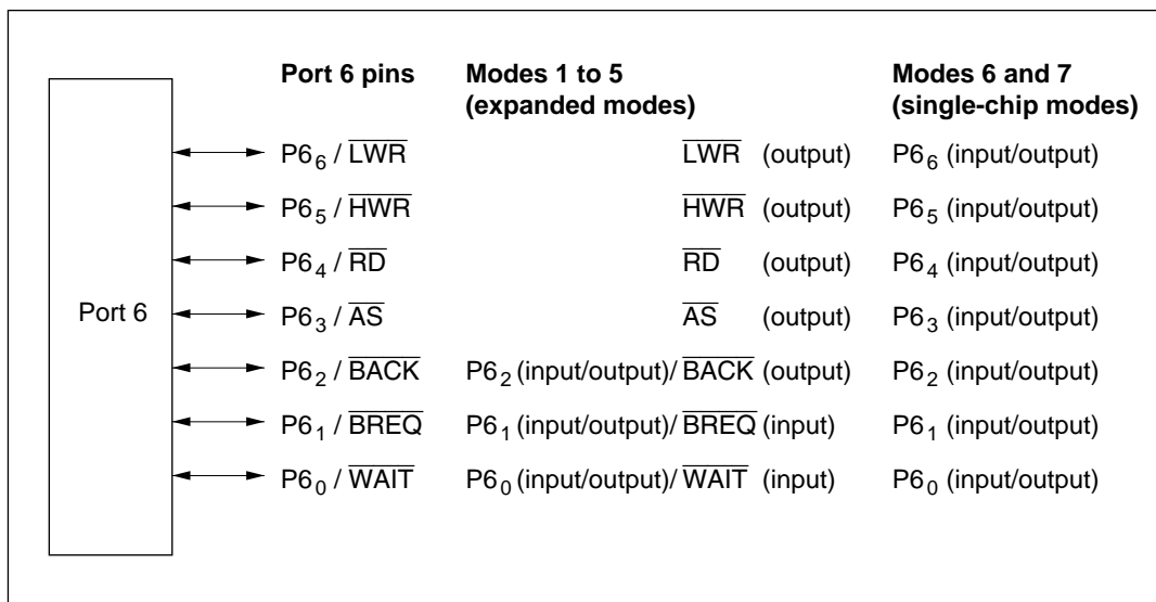
Figure 9-20 Port 6 Pin Configuration
