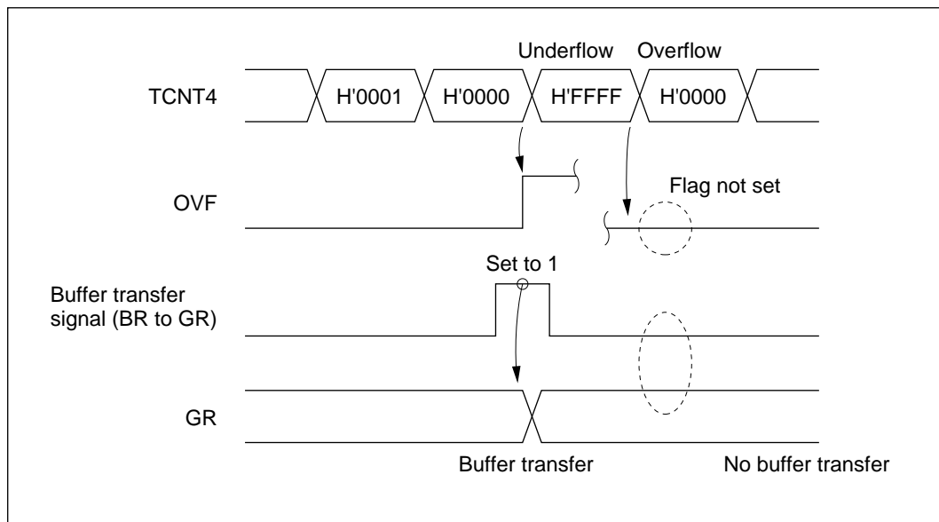
Figure 10-38 Undershoot Timing
