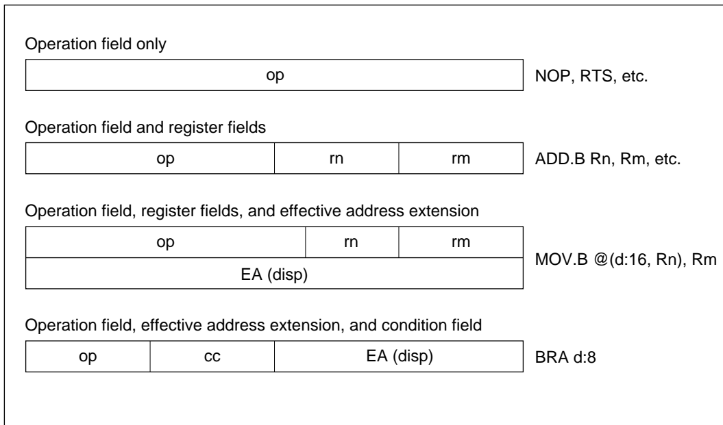
Figure 2-9 Instruction Formats
