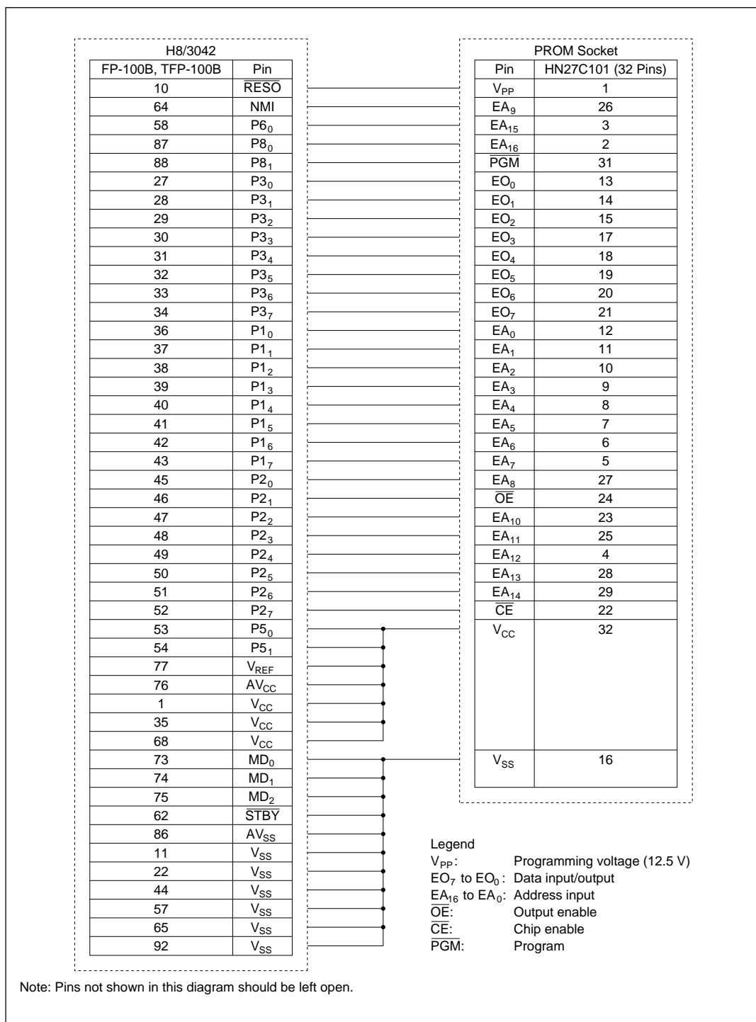
Figure 17-2 Socket Adapter Pin Assignments
