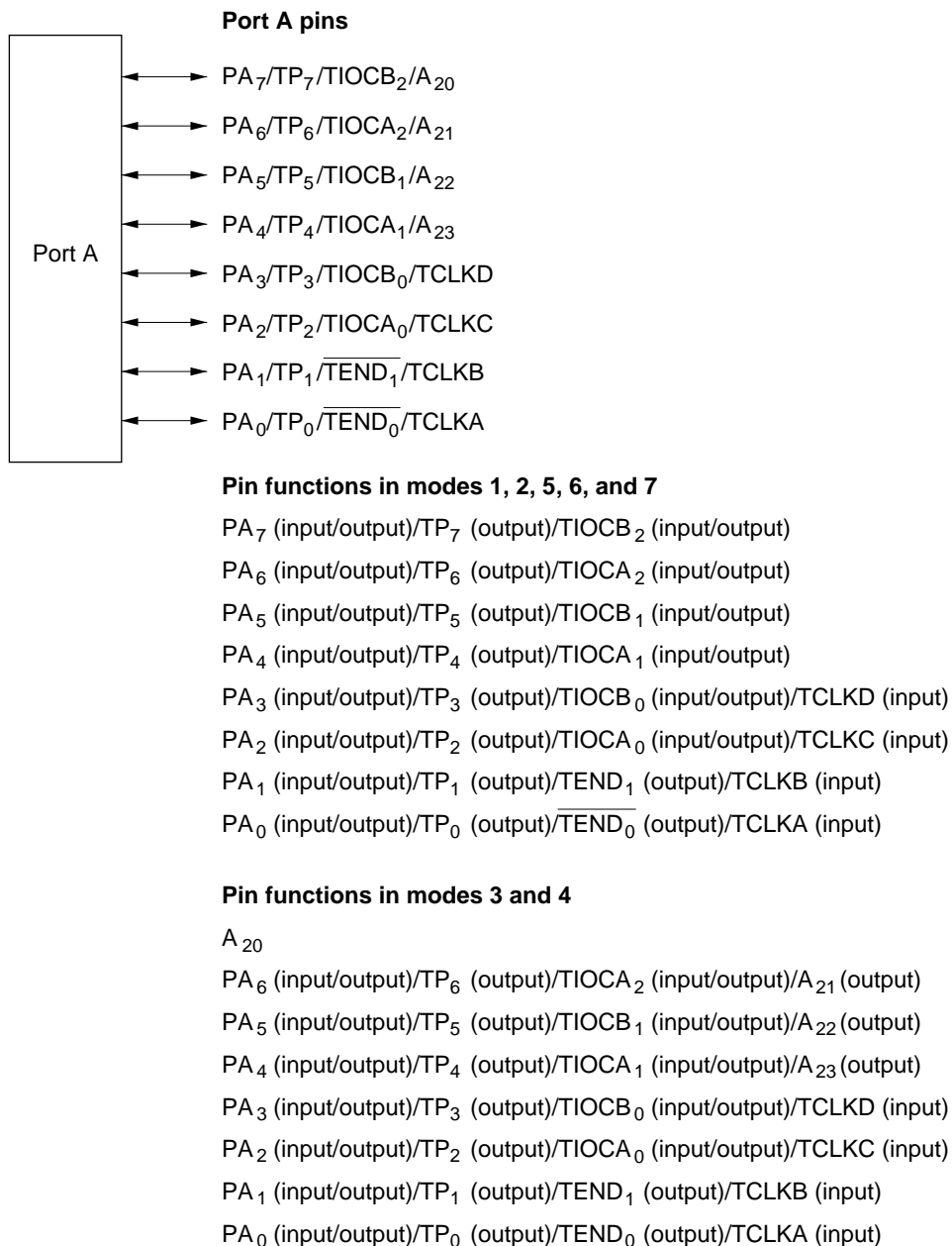
Figure 9-28 Port A Pin Configuration
