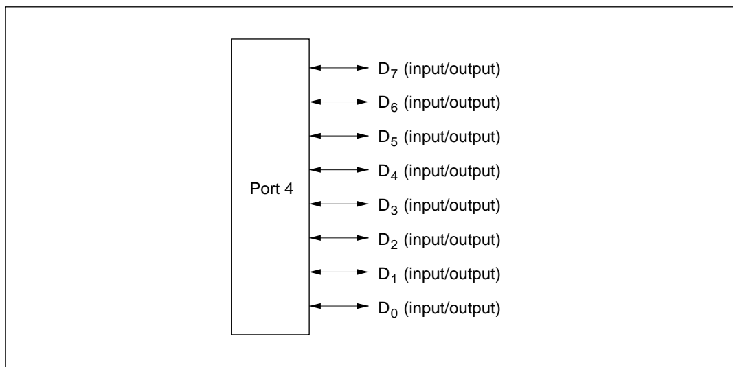
Figure 9-14 Pin Functions in 16-Bit Bus Mode (Port 4)
