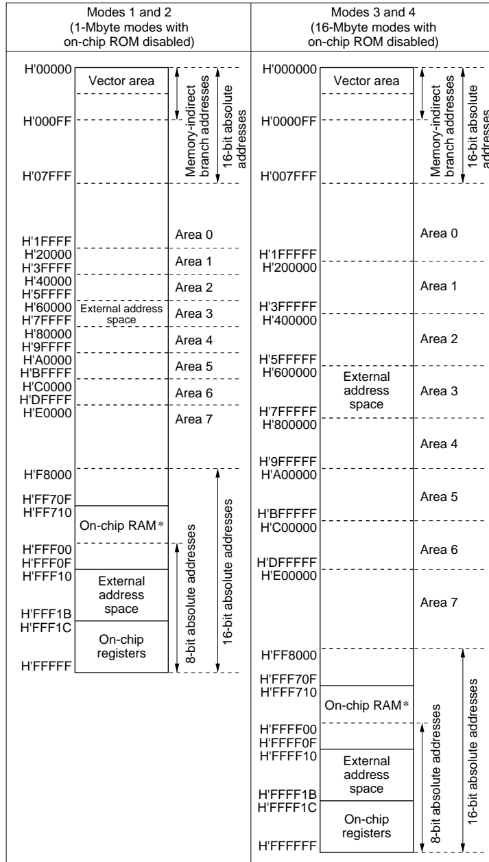
Figure 3-1 H8/3042 Memory Map in Each Operating Mode (1)
