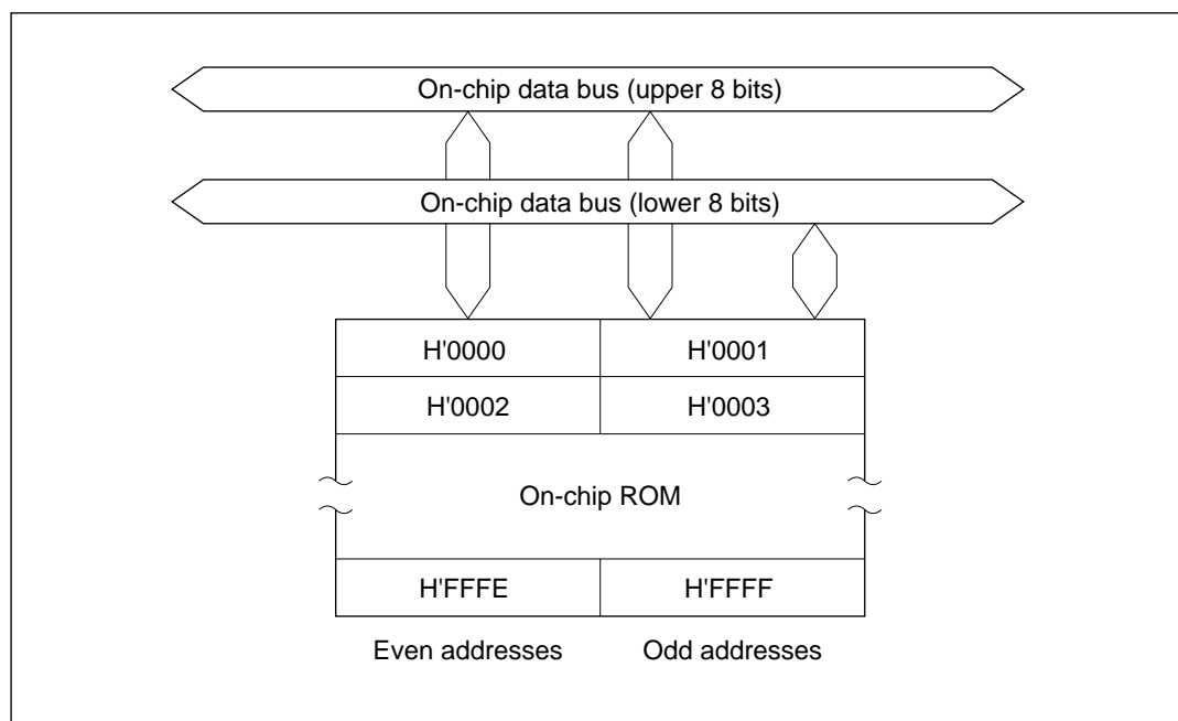
Figure 17-1 ROM Block Diagram (H8/3042)
