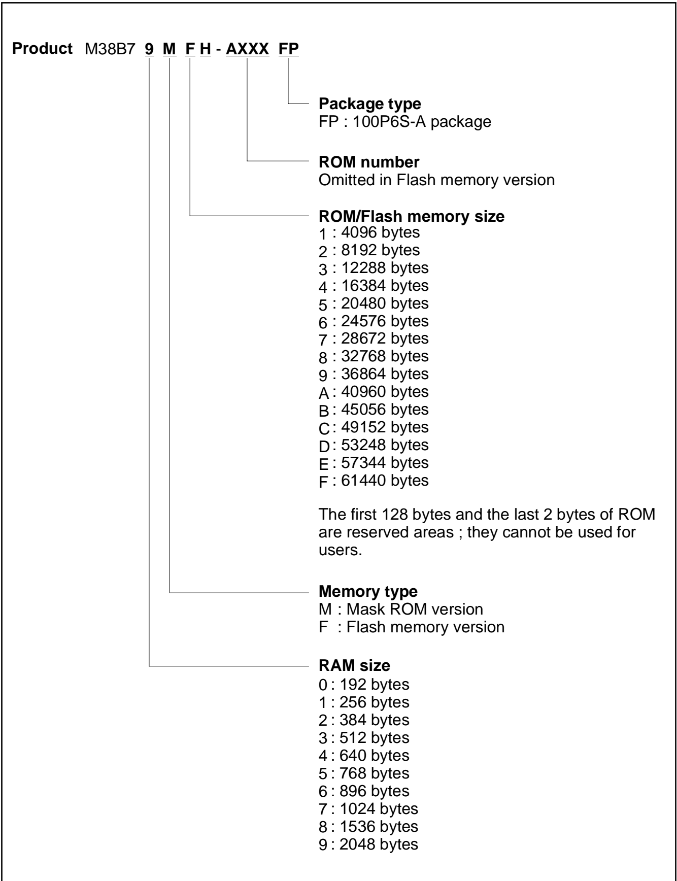
Fig. 3 Part numbering
