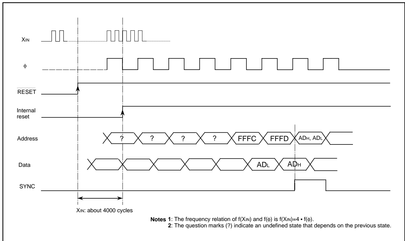
Fig. 77 Reset sequence
