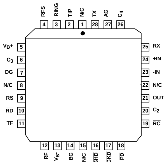
HC-5504B (PLCC) TOP VIEW
