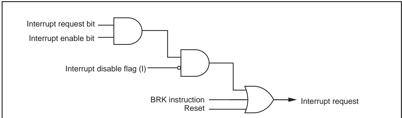
Fig. 9 Interrupt control
