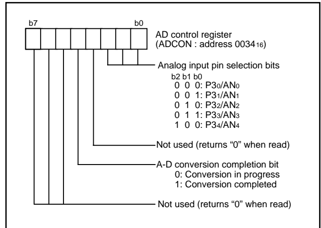
Fig. 36 Structure of AD control register
