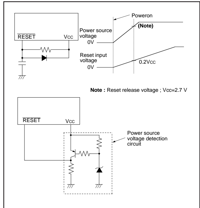
Fig. 41 Reset circuit example
