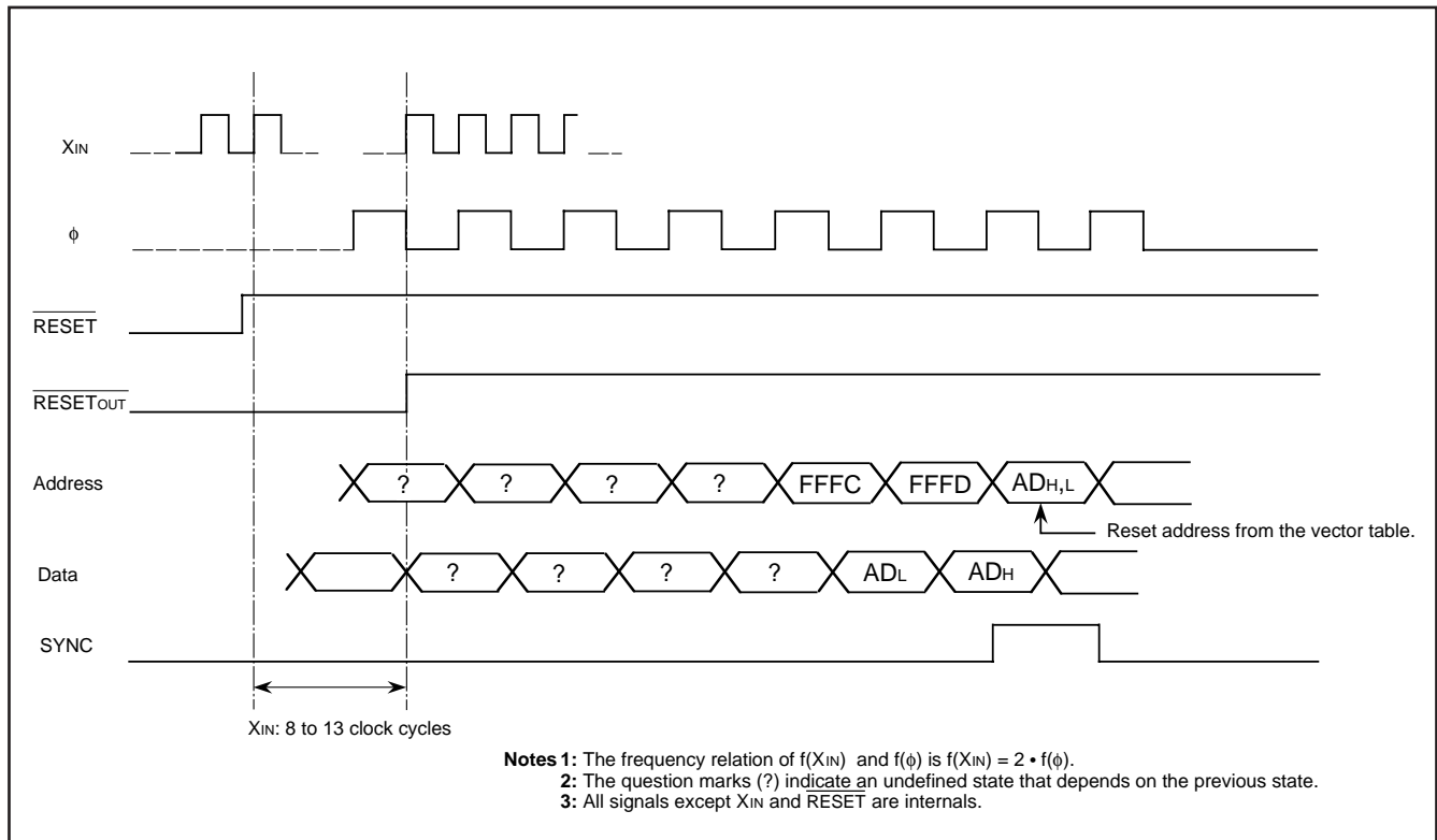
Fig. 42 Reset sequence
