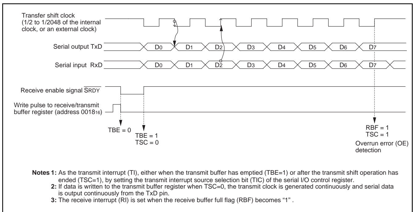
Fig. 15 Operation of clock synchronous serial I/O function
