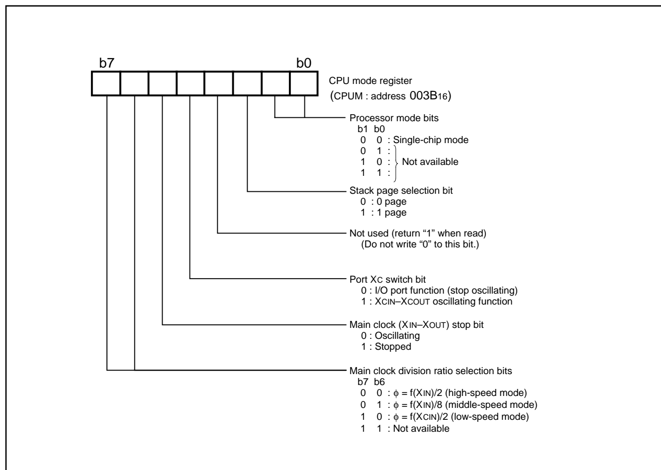
Fig. 4 Structure of CPU mode register
