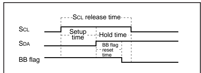
Fig. 29 STOP condition detecting timing diagram
