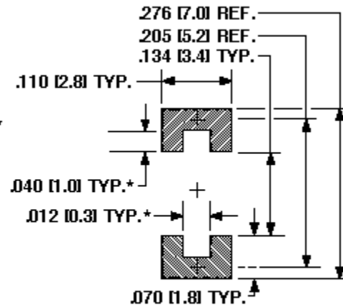
PAD LAYOUT
