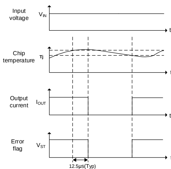
Figure 19. BD1HD500 BD1HDU50 Self-restart Overheat Protection Timing Chart
