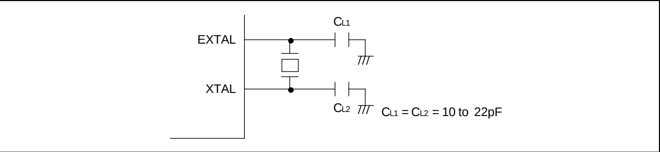
Figure 16-2. Connection of Crystal Oscillator (Example)
