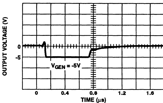
7G. V_{OUT} vs TIME
