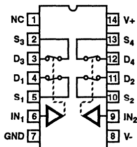
DUAL DPST HI-302 AND HI-306 (PDIP, CDIP, SOIC)
