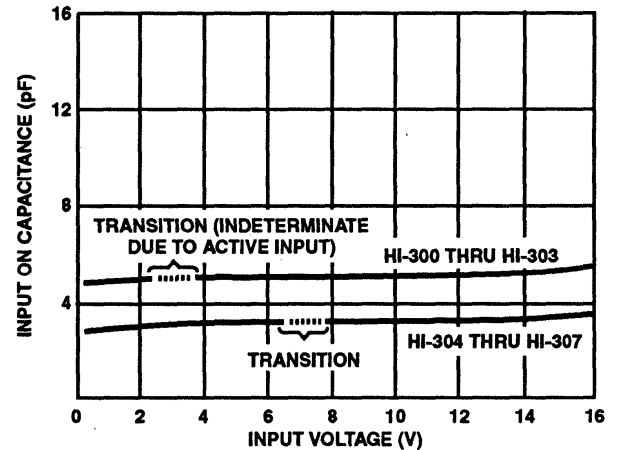
FIGURE 9. DIGITAL INPUT CAPACITANCE vs INPUT VOLTAGE
