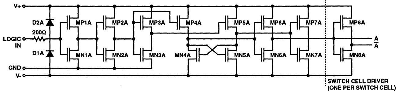
DIGITAL INPUT BUFFER AND LEVEL SHIFTER
