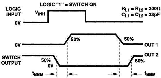
FIGURE 18. BREAK-BEFORE-MAKE TEST CIRCUIT ( t_{BBM} )
