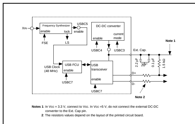
Fig.112 Peripheral circuit
