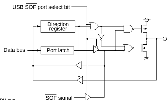
(12) Port P70
