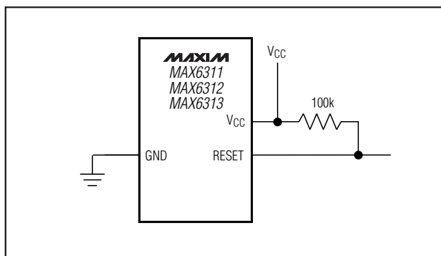
Figure 5. Ensuring RESET Valid to V_{CC} = 0V
