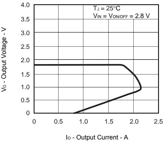
V_O vs. I_O ( \mu PD121W18A)
