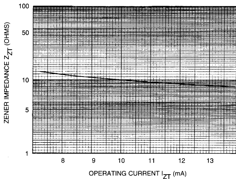
TYPICAL CHANGE OF ZENER IMPEDANCE WITH CHANGE IN OPERATING CURRENT
