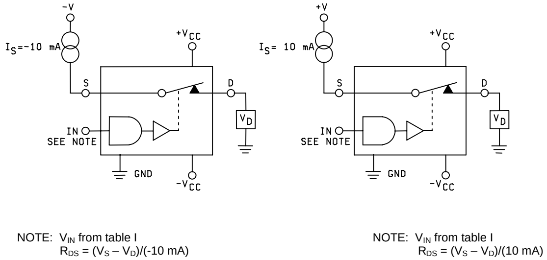
Figure 4. R_{DS} test circuits.
