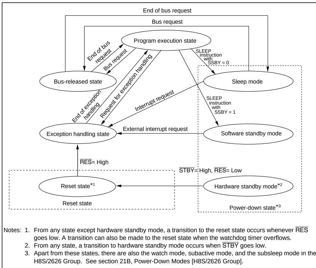
Figure 2.15 State Transitions
