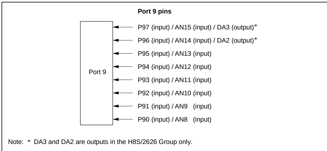
Figure 9.3 Port 9 Pin Functions
