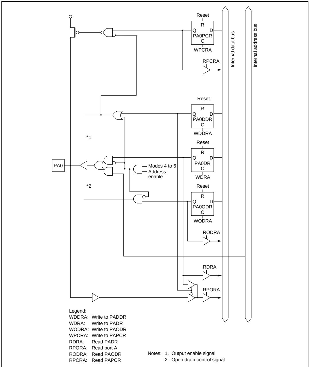
Figure C.4 (a) Port A Block Diagram (Pin PA0)
