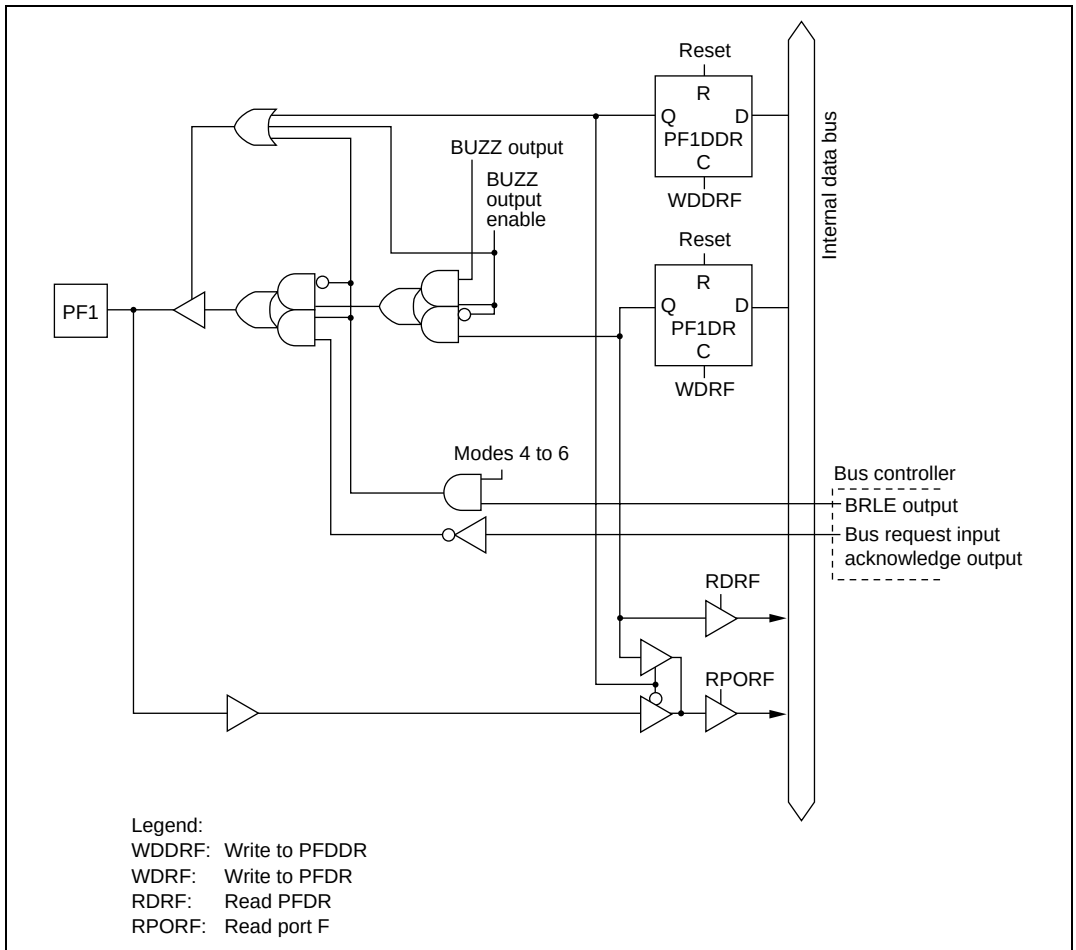
Figure C.9 (c) Port F Block Diagram in the H8S/2626 Group (Pin PF1)
