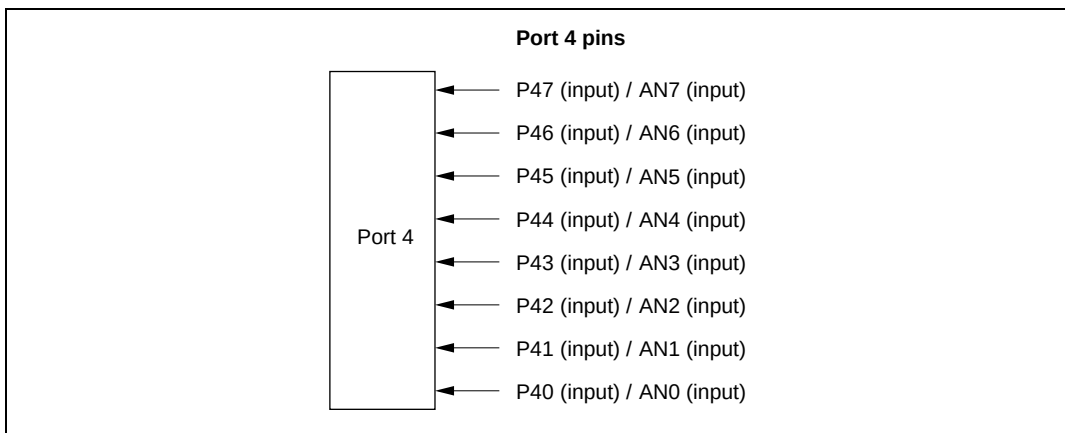
Figure 9.2 Port 4 Pin Functions
