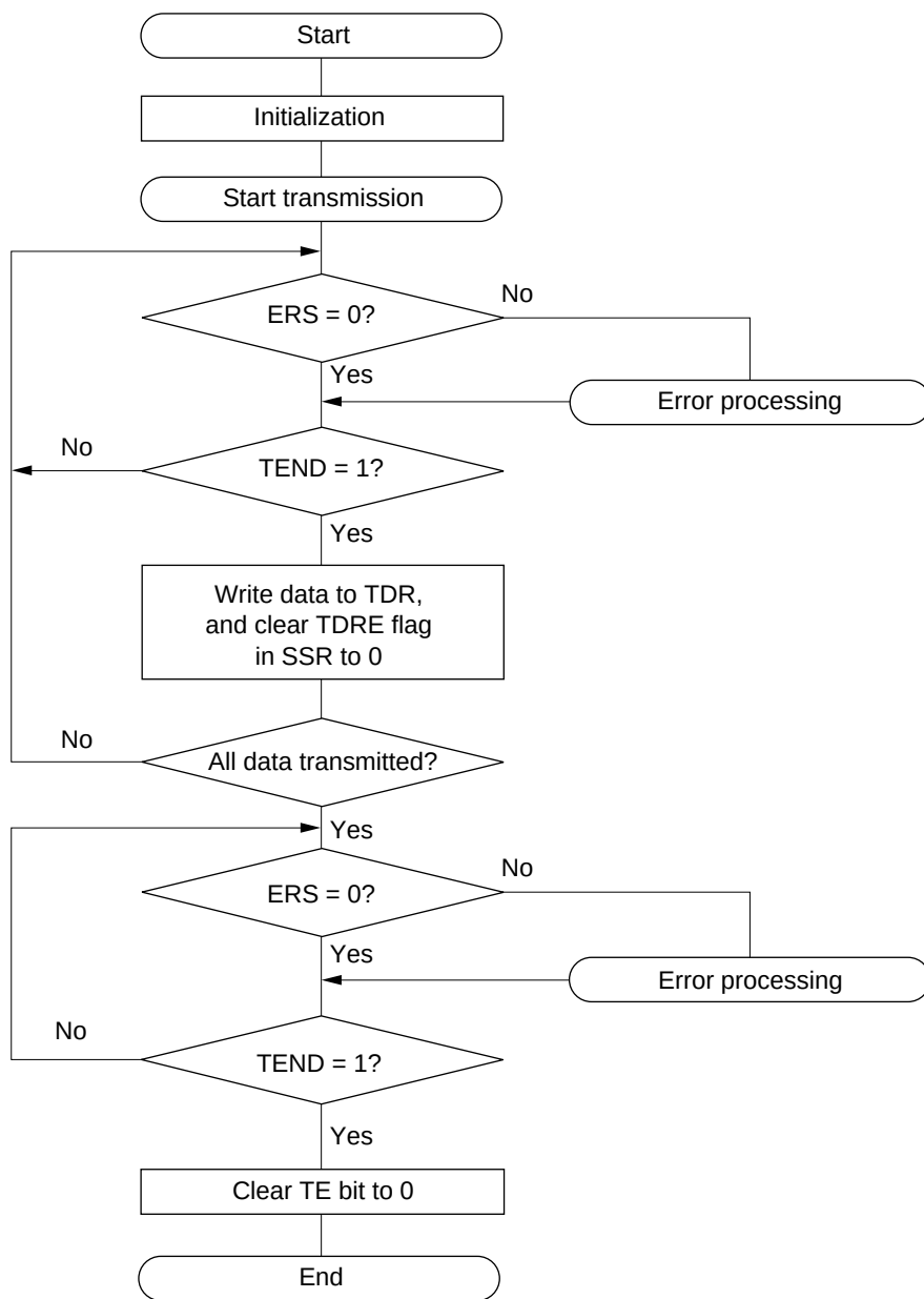
Figure 14.4 Example of Transmission Processing Flow
