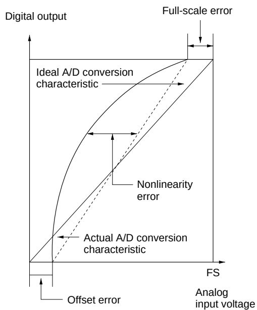
Figure 16.10 A/D Conversion Precision Definitions (2)
