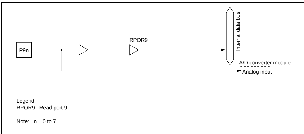
Figure C.3 Port 9 Block Diagram (Pins P90 to P97)
