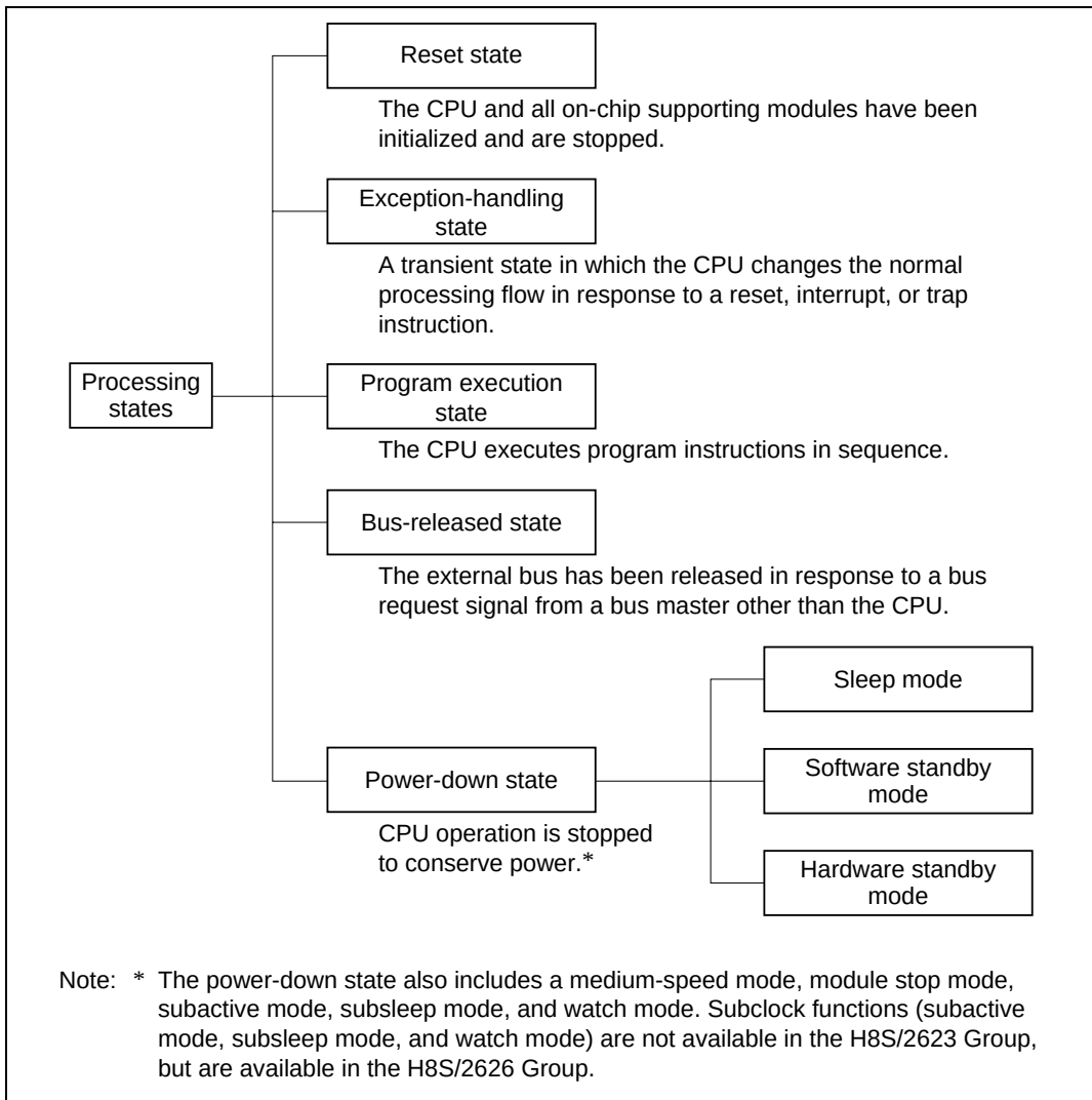
Figure 2.14 Processing States
