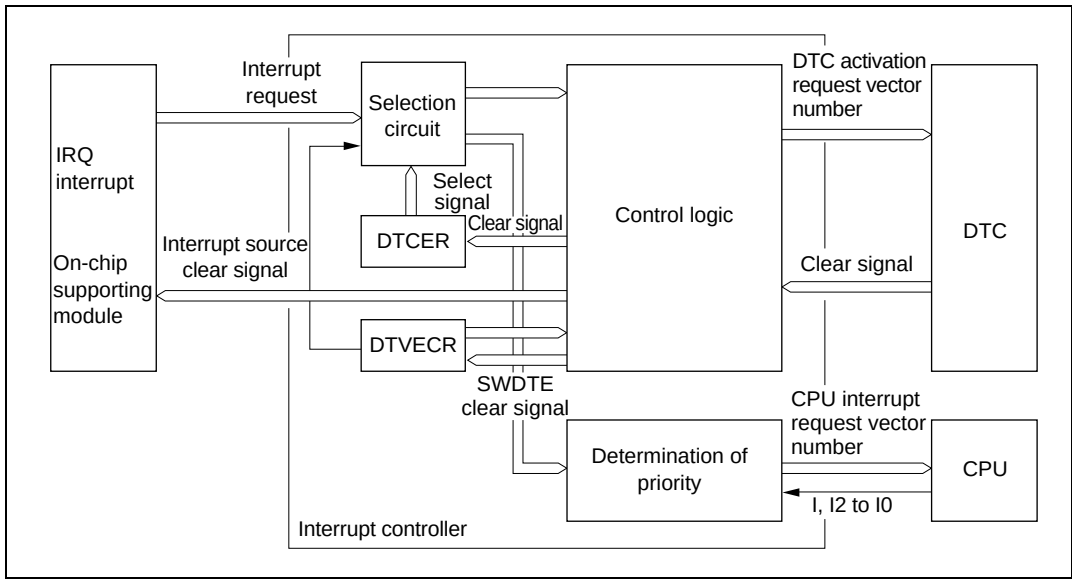
Figure 5.9 Interrupt Control for DTC
