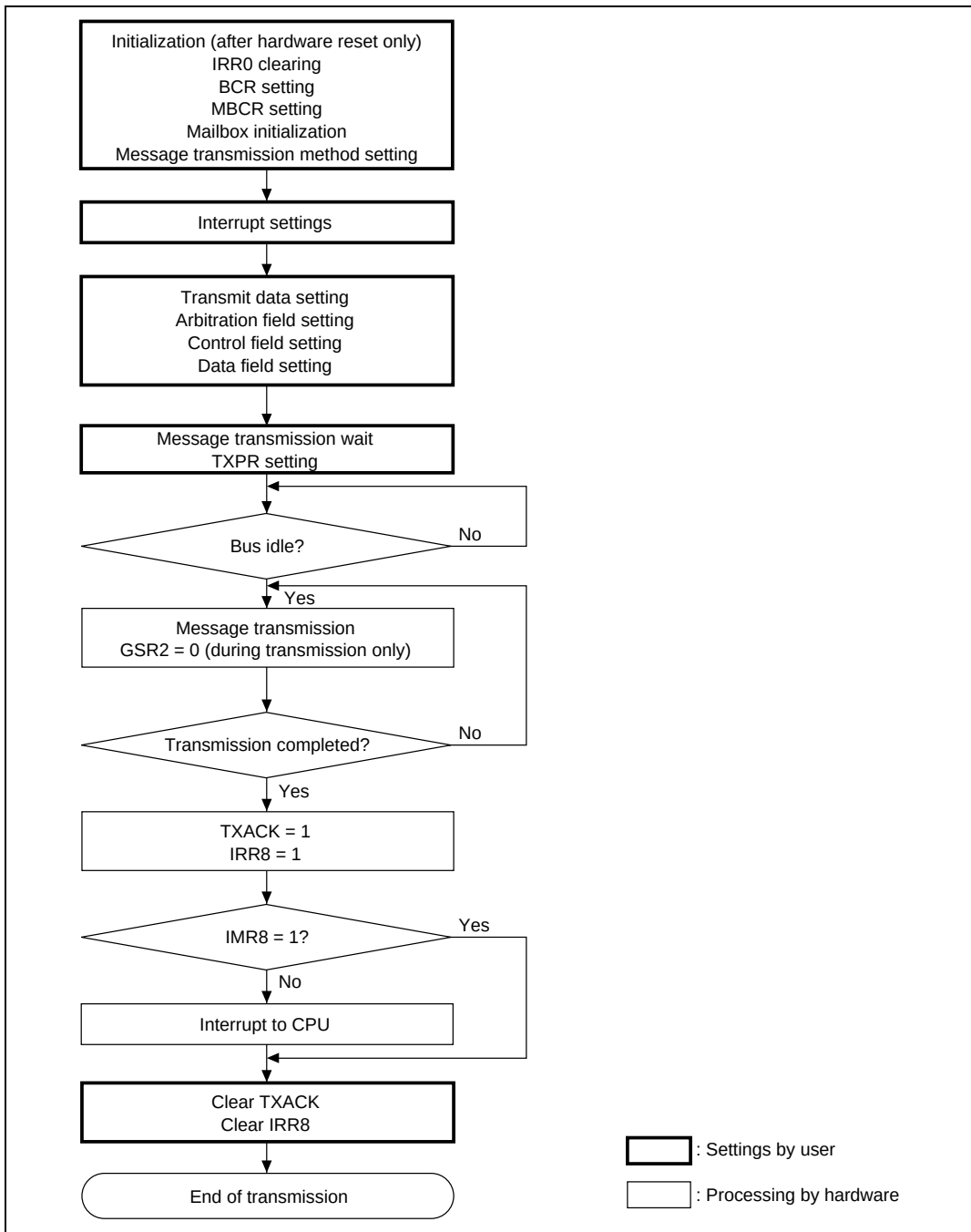
Figure 15.7 Transmission Flowchart
