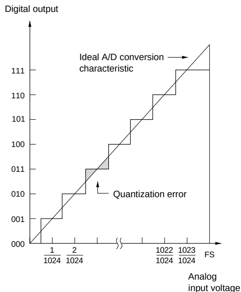
Figure 16.9 A/D Conversion Precision Definitions (1)
