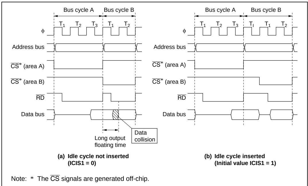
Figure 7.15 Example of Idle Cycle Operation (1)
