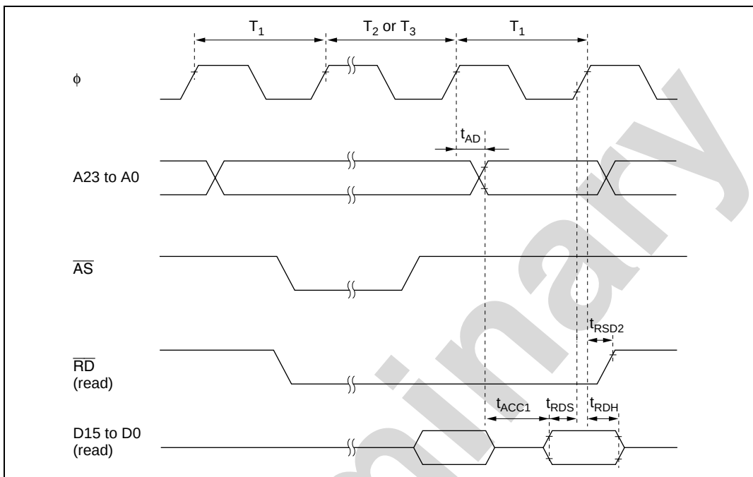
Figure 22.10 Burst ROM Access Timing (One-State Access)
