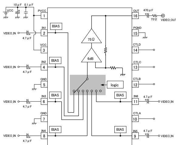
Fig.8 BH76361FV
