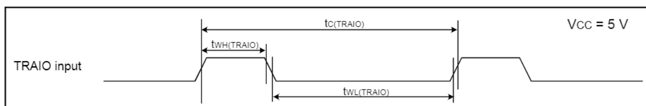
Figure 21.9 TRAIO Input and \overline{INT1} Input Timing Diagram when V_{CC} = 5\text{ V}
