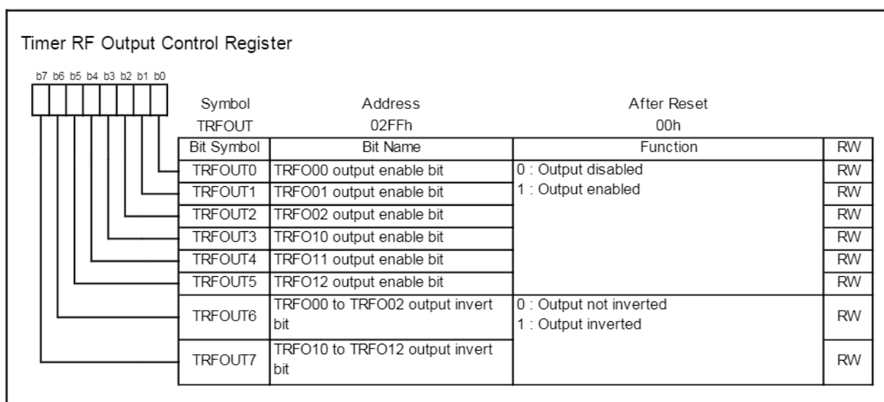
Figure 14.180 TRFOUT Register
