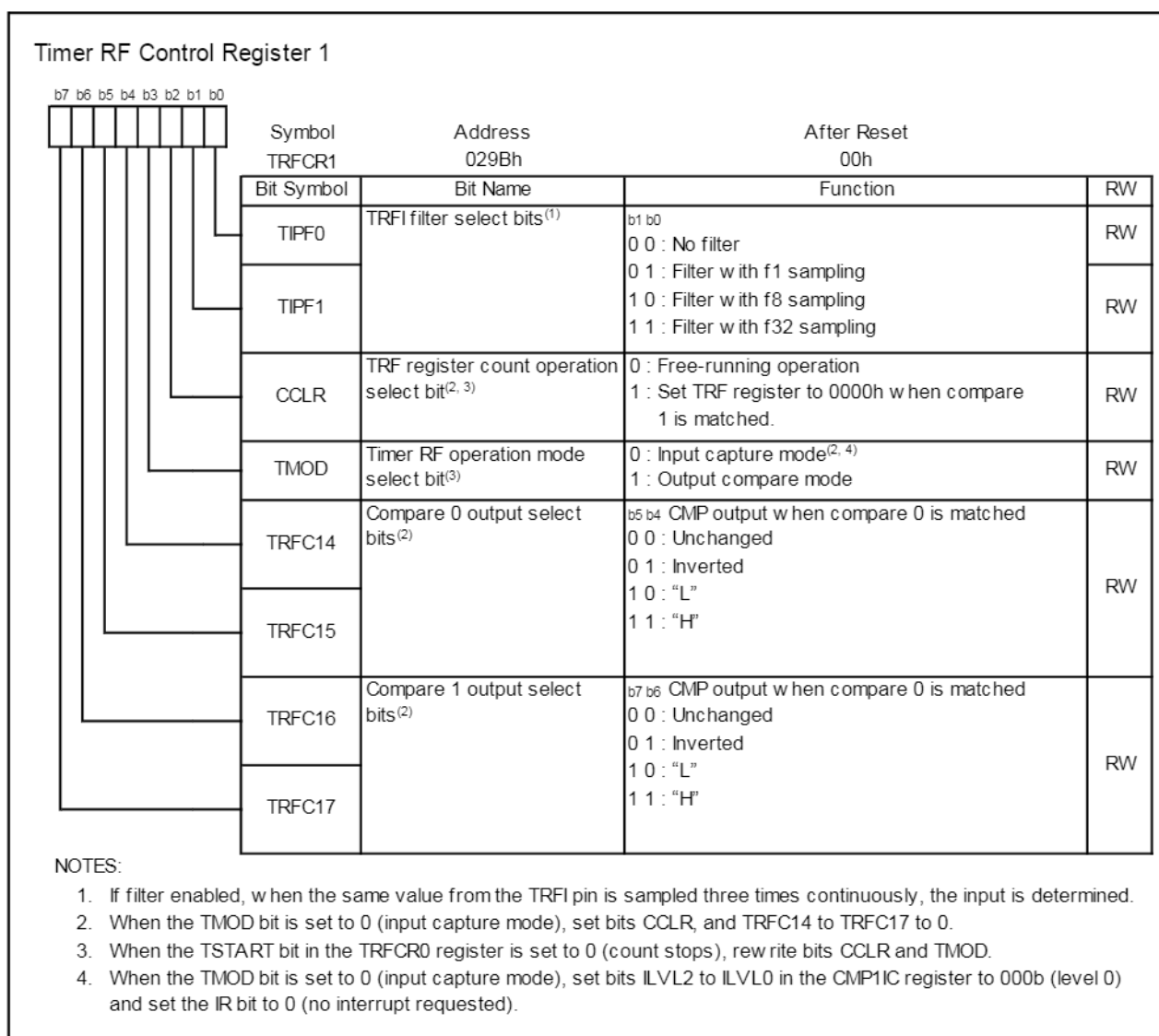
Figure 14.179 TRFCR1 Register
