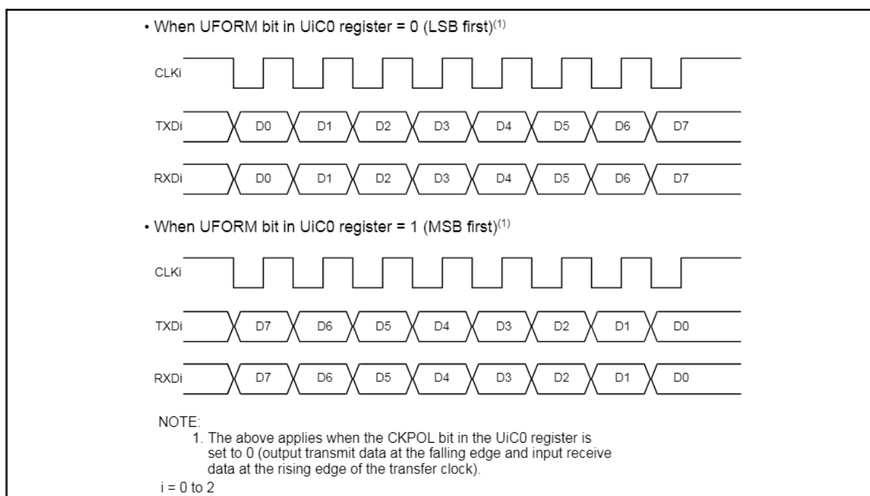
Figure 15.11 Transfer Format
