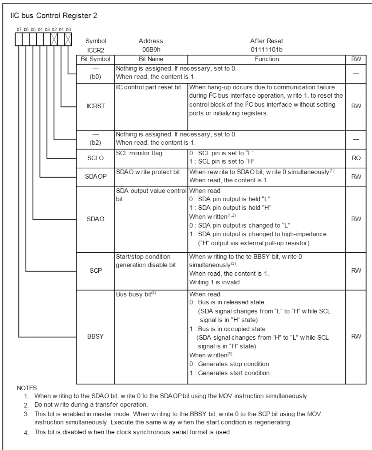
Figure 16.27 ICCR2 Register
