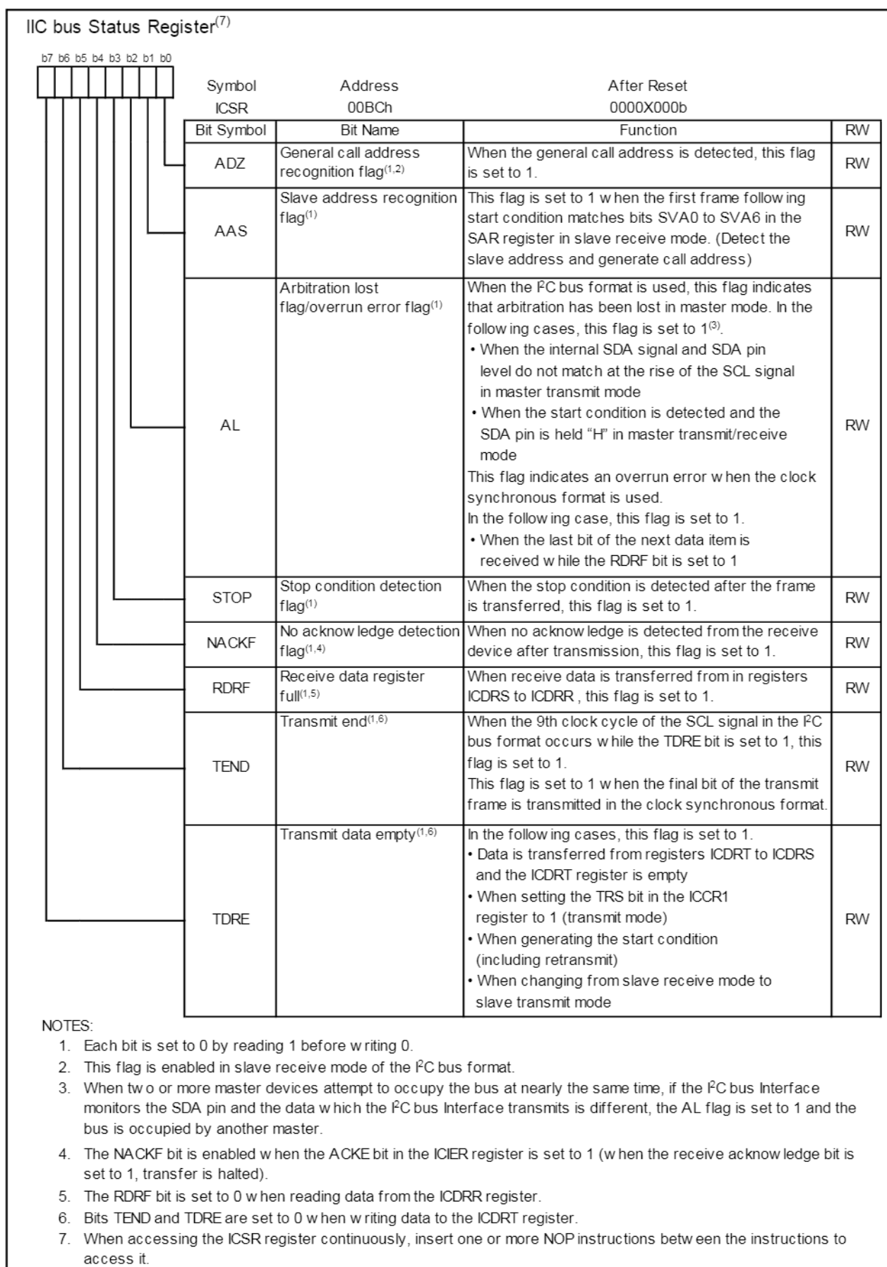
Figure 16.30 ICSR Register
