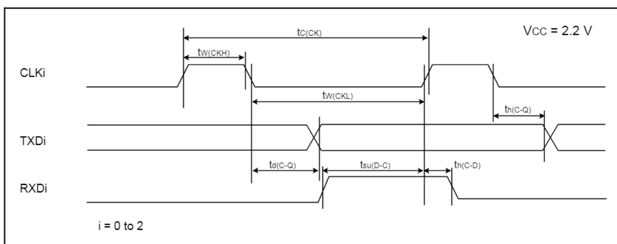
Figure 21.21 Serial Interface Timing Diagram when V_{CC} = 2.2 \text{ V}
