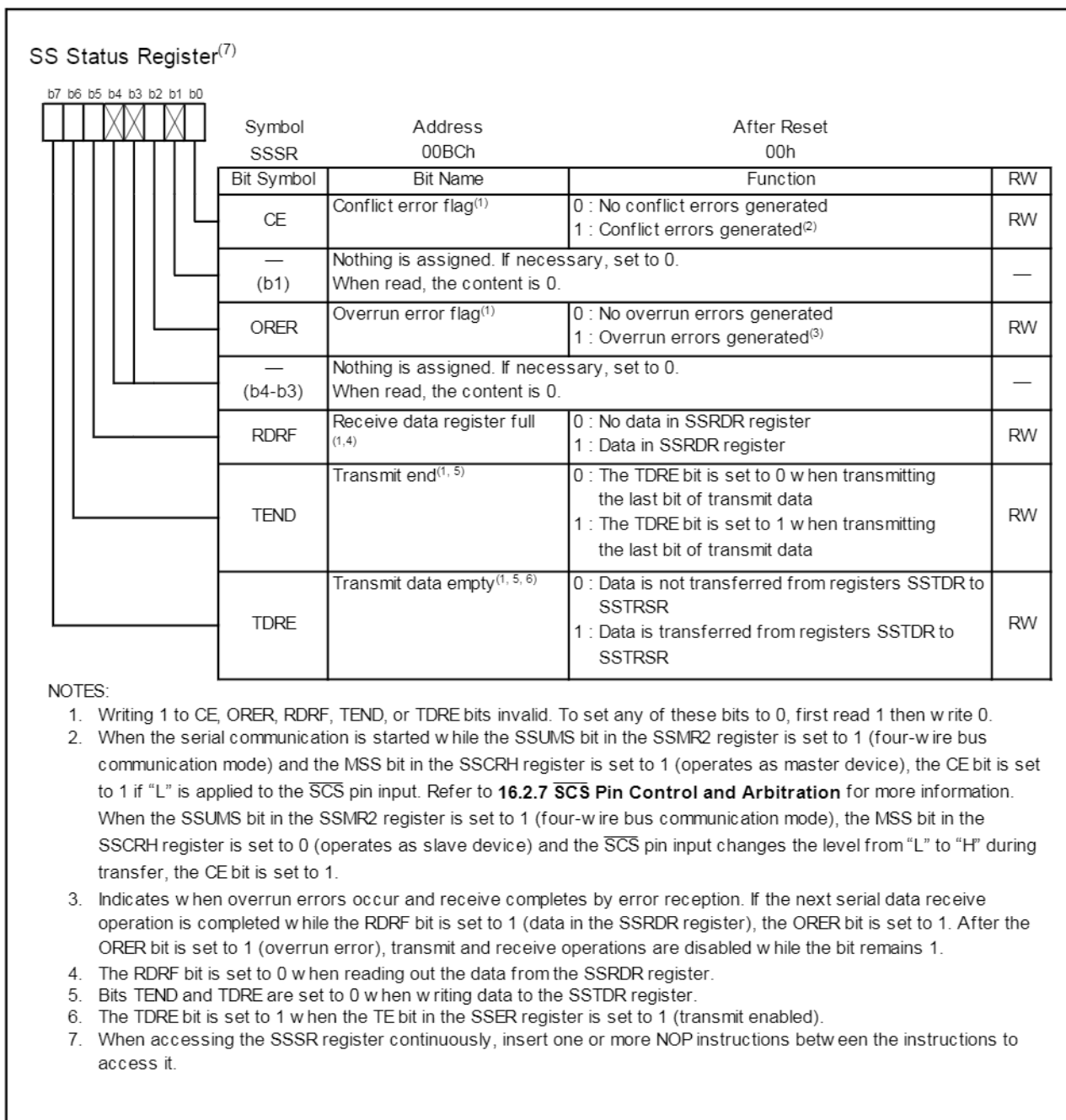
Figure 16.7 SSSR Register
