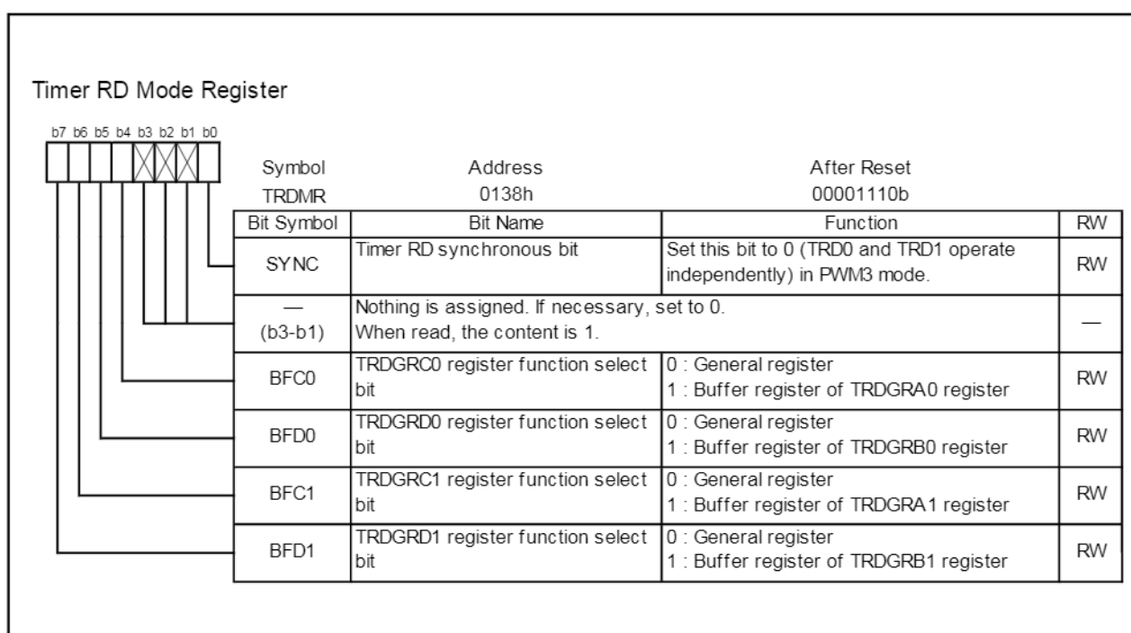
Figure 14.141 TRDMR Register in PWM3 Mode
