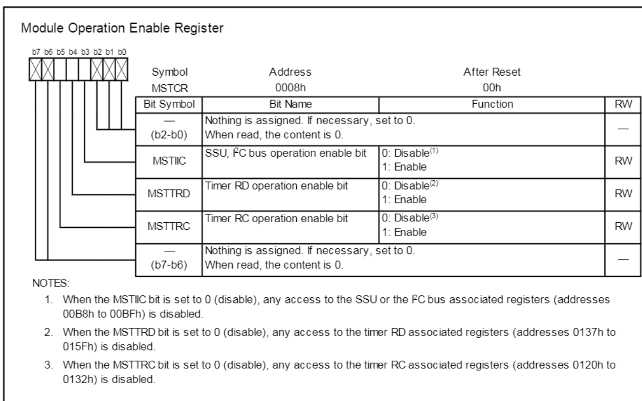
Figure 14.27 MSTCR Register
