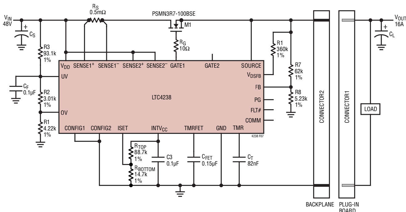
Figure 7. 48V, 16A A Single MOSFET Implementation with HSSS Mode
