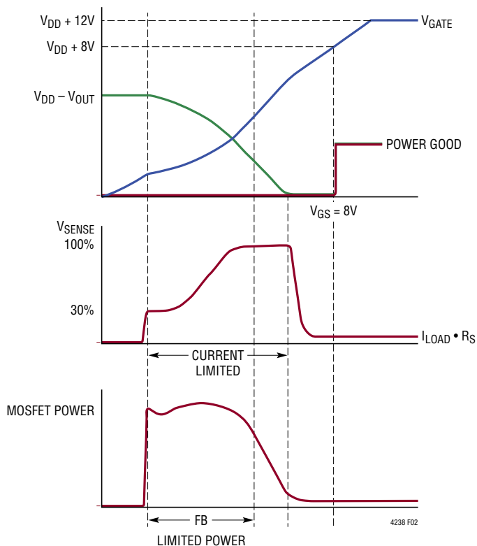
Figure 2. Power-Up Waveforms
