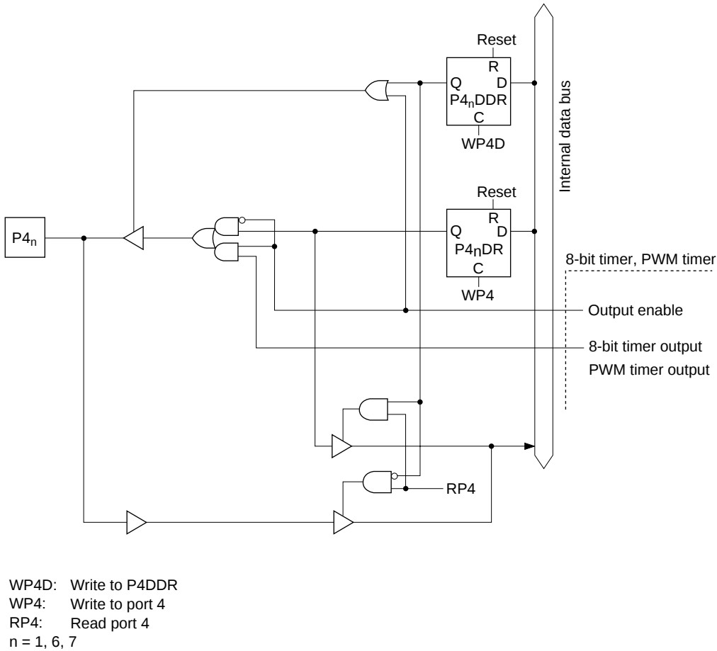
Figure C.4 (b) Port 4 Block Diagram (Pins P4_1 , P4_6 , P4_7 )
