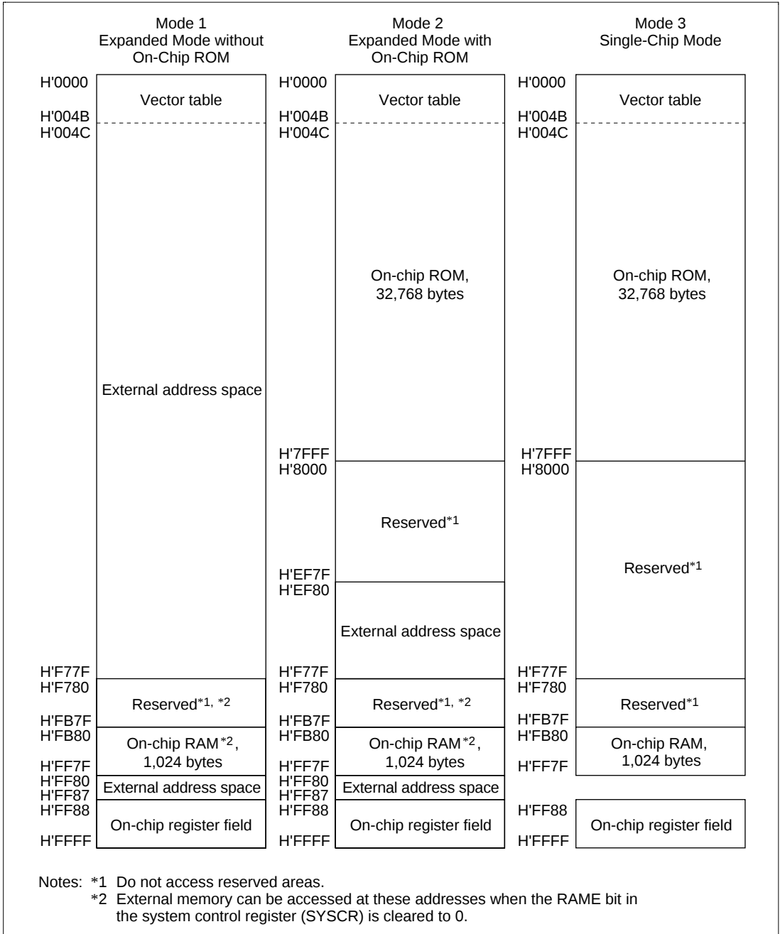
Figure 3.3 H8/3334Y, H8/3394 Address Space Map
