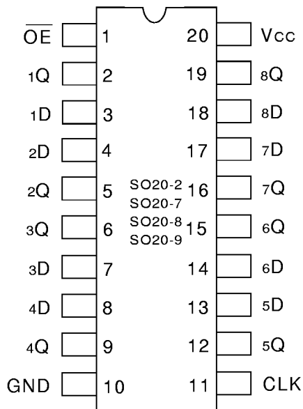
SOIC/ SSOP/ QSOP/ TSSOP TOP VIEW
