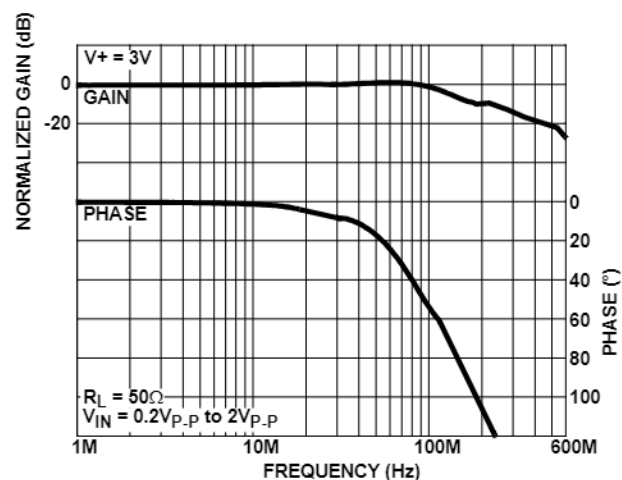
FIGURE 19. FREQUENCY RESPONSE
