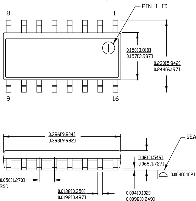
Figure 10. 16-Pin (150-Mil) SOIC (51-85068)
