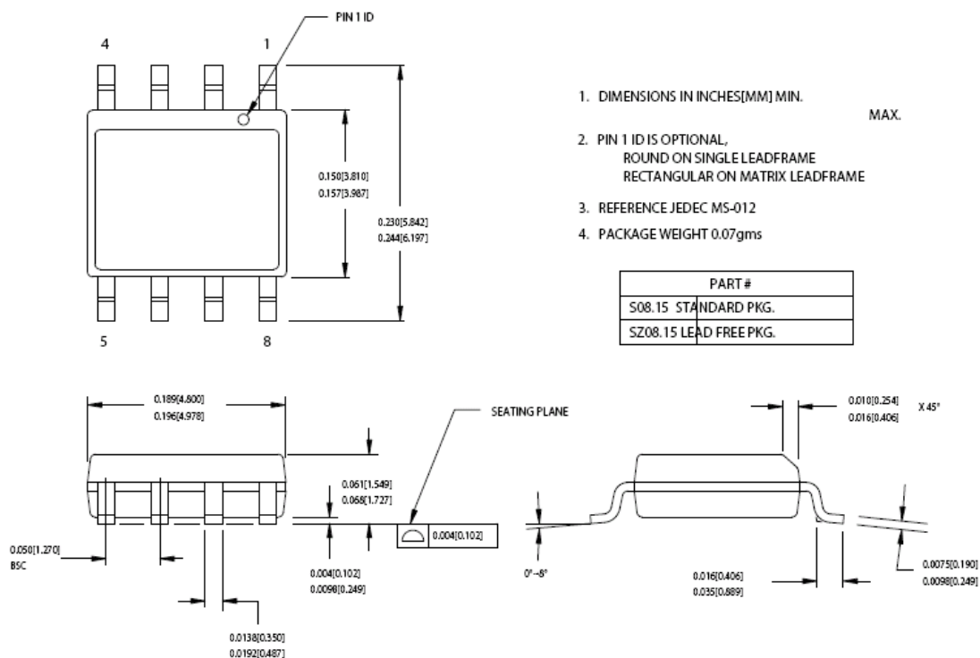
Figure 11. 8-Pin (150-Mil) SOIC (51-85066)
