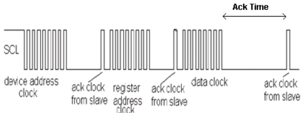
Figure 5. Read ACK Time Representation [3]
