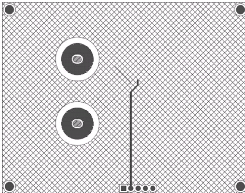
Figure 6. Top Layer
