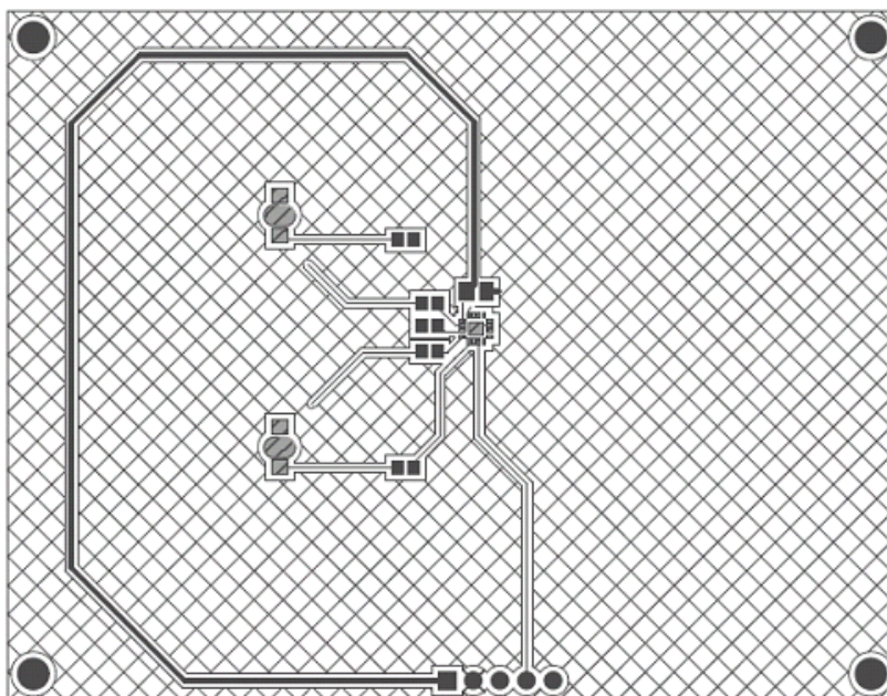
Figure 7. Bottom Layer
