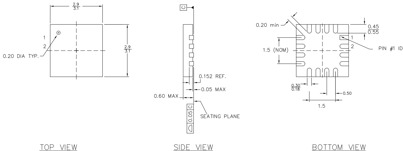
Figure 9. 16-Pin Chip On Lead 3 X 3 mm (Sawn) (001-09116)
