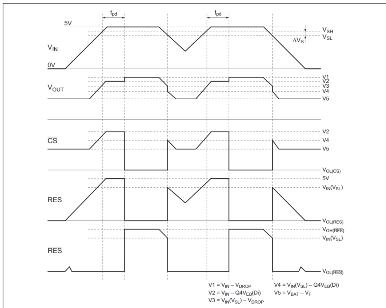
Figure 6 Timing Chart
