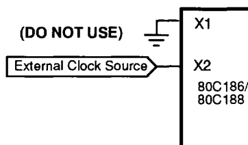
Figure 6. 80C186/C188 Oscillator Configurations
