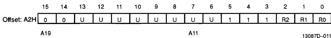
Figure 10. LMCS Register
