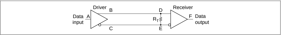
Figure 8 1 : 1 Unidirectional Transmission
