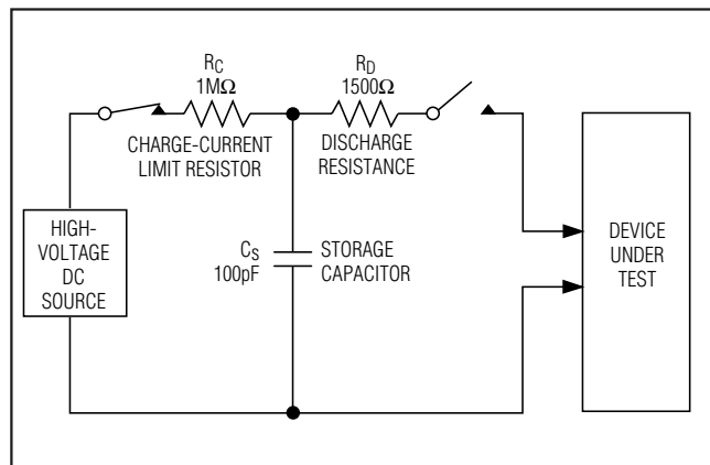
Figure 31a. Human Body ESD Test Model
