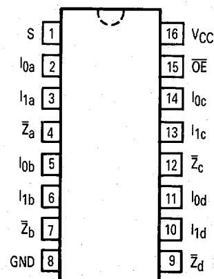
CONNECTION DIAGRAM
