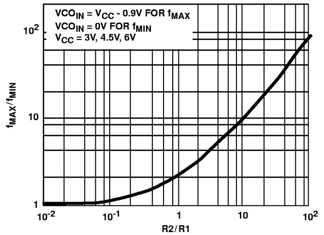
FIGURE 33. HC7046A f_{MIN}/f_{MAX} vs R2/R1
