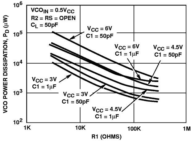
FIGURE 42. HC7046A VCO POWER DISSIPATION vs R_1 ( C_1 = 50\text{pF}, 1\mu\text{F} )
