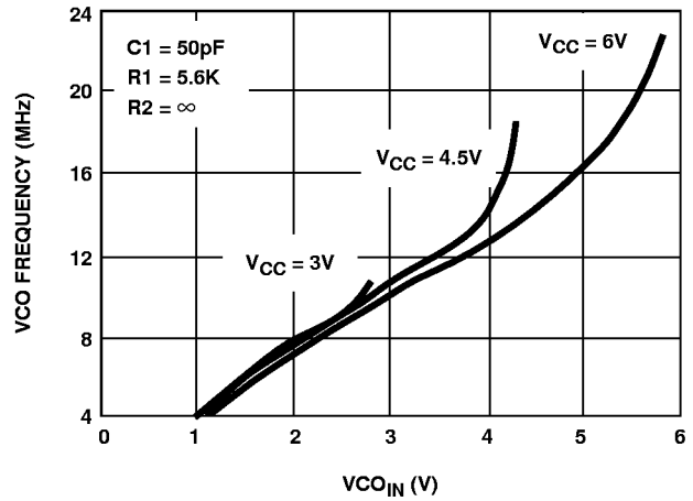
FIGURE 23. HC7046A TYPICAL VCO FREQUENCY vs V_{CO\_IN} ( R_1 = 5.6k\Omega , C_1 = 50pF )
