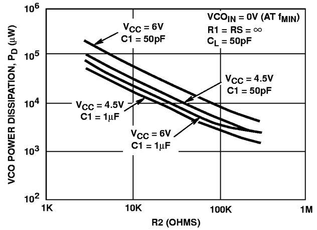
FIGURE 43. HCT7046A VCO POWER DISSIPATION vs R_2 ( C_1 = 50\text{pF}, 1\mu\text{F} )
