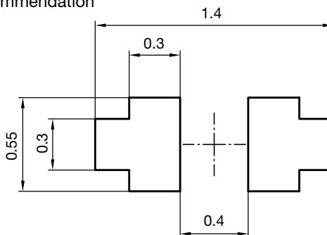
Footprint recommendation
