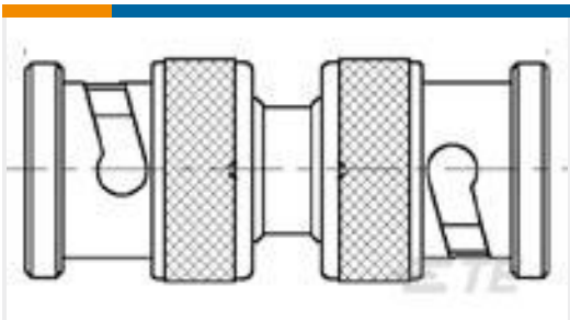
TE Part # 1-1478043-0 BNC M TO BNC M ADAPTOR,STR,75 OHM,2G
