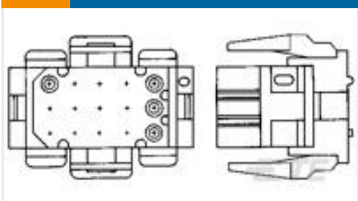
TE Part # 1-640521-0 09P MR II PLUG HSG V0
