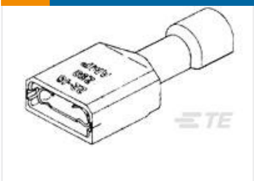
TE Part # 2-520409-2 ULTRA-FAST 187 ASY REC 22-18 TPBR
