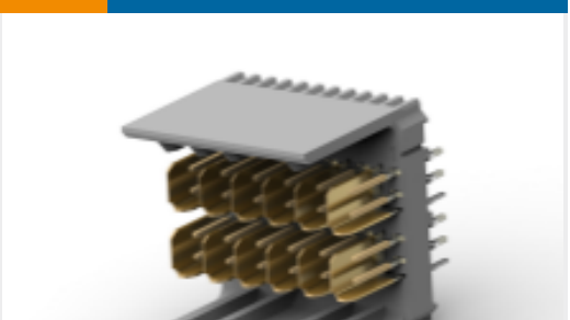
TE Part # 2274610-1 HM-ZD 2PR HDR 24P 2.5MM
